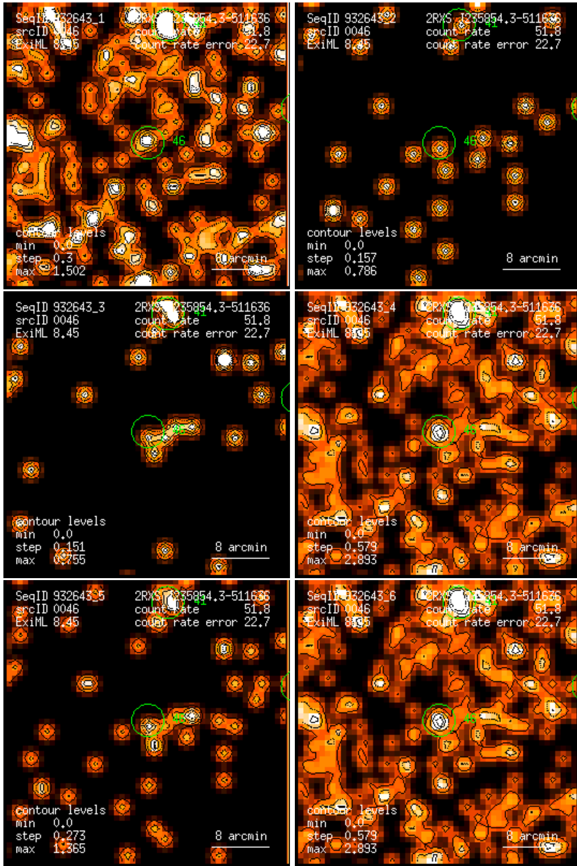
Figure 46: RASS 932643: detection 0046: band rate images, Gaussian filter: (1) PSPC channels 11 – 41, (2) 52 – 90, (3) 91 – 201, (4) 11 – 235, (5) 52 – 201, (6) 11 – 201. Broad band rates in counts/ks. Band rate contour levels in counts/ks/arcmin 2 .
