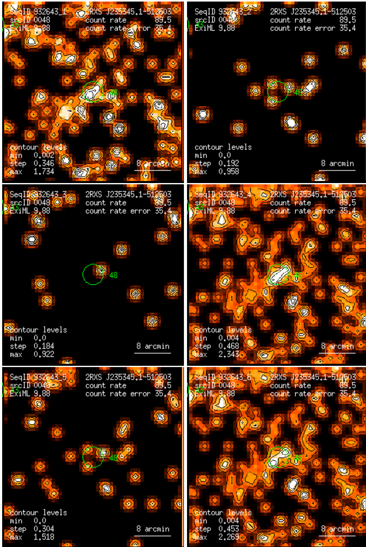
Figure 48: RASS 932643: detection 0048: band rate images, Gaussian filter: (1) PSPC channels 11 – 41, (2) 52 – 90, (3) 91 – 201, (4) 11 – 235, (5) 52 – 201, (6) 11 – 201. Broad band rates in counts/ks. Band rate contour levels in counts/ks/arcmin 2 .
