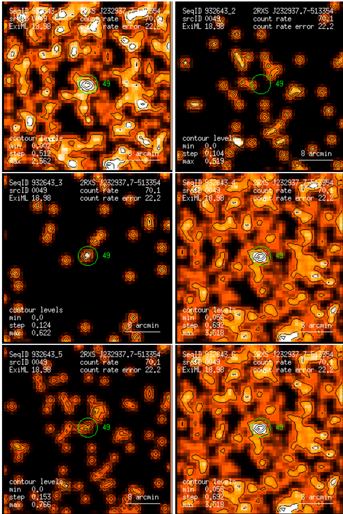
Figure 49: RASS 932643: detection 0049: band rate images, Gaussian filter: (1) PSPC channels 11 – 41, (2) 52 – 90, (3) 91 – 201, (4) 11 – 235, (5) 52 – 201, (6) 11 – 201. Broad band rates in counts/ks. Band rate contour levels in counts/ks/arcmin 2 .
