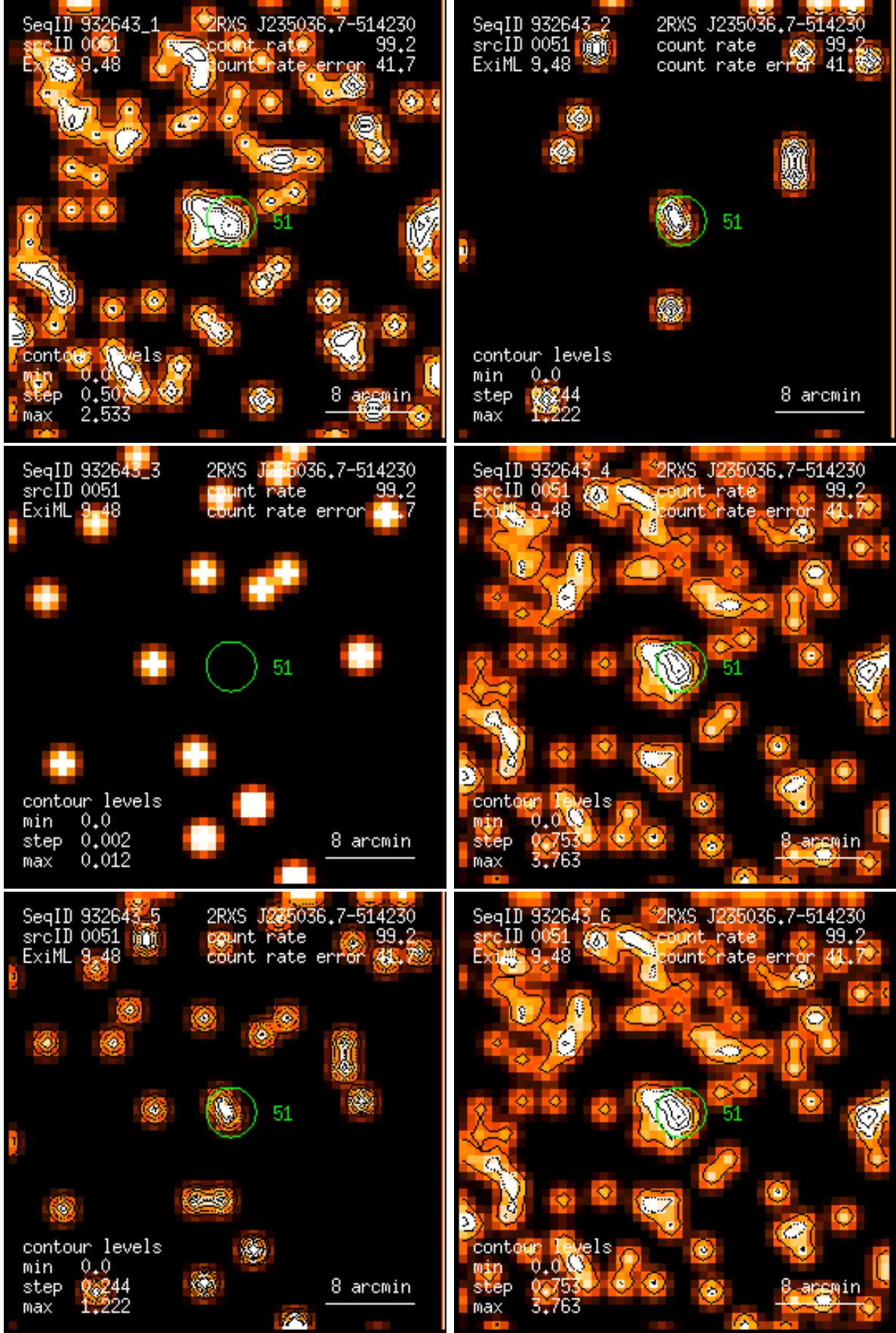
Figure 51: RASS 932643: detection 0051: band rate images, Gaussian filter: (1) PSPC channels 11 – 41, (2) 52 – 90, (3) 91 – 201, (4) 11 – 235, (5) 52 – 201, (6) 11 – 201. Broad band rates in counts/ks. Band rate contour levels in counts/ks/arcmin 2 .
