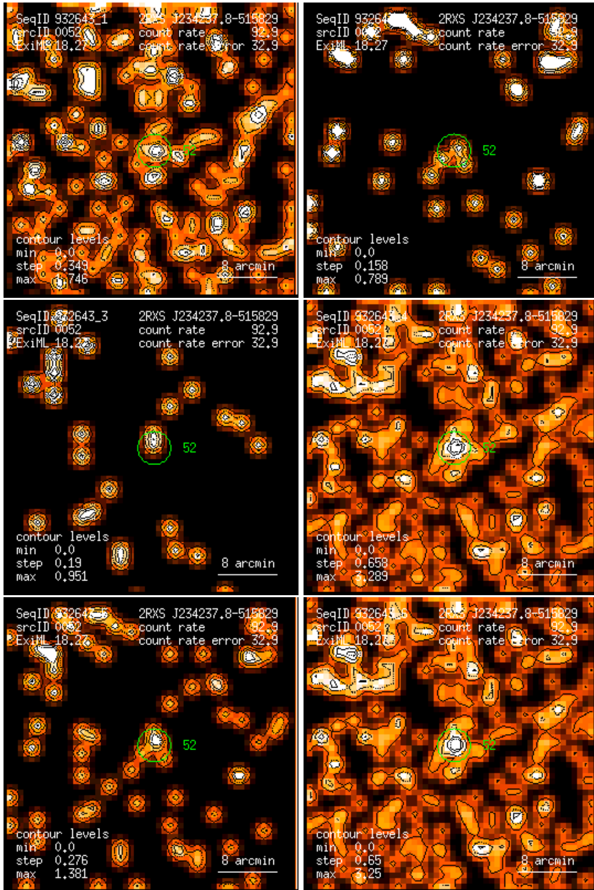
Figure 52: RASS 932643: detection 0052: band rate images, Gaussian filter: (1) PSPC channels 11 – 41, (2) 52 – 90, (3) 91 – 201, (4) 11 – 235, (5) 52 – 201, (6) 11 – 201. Broad band rates in counts/ks. Band rate contour levels in counts/ks/arcmin 2 .
