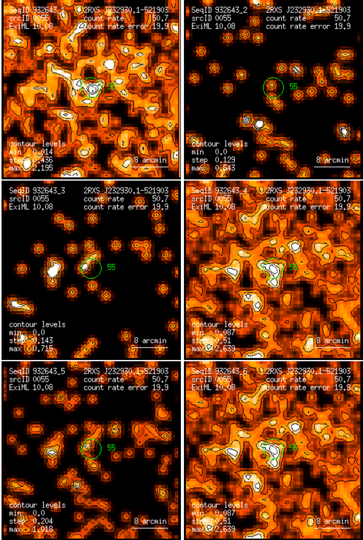
Figure 55: RASS 932643: detection 0055: band rate images, Gaussian filter: (1) PSPC channels 11 – 41, (2) 52 – 90, (3) 91 – 201, (4) 11 – 235, (5) 52 – 201, (6) 11 – 201. Broad band rates in counts/ks. Band rate contour levels in counts/ks/arcmin 2 .
