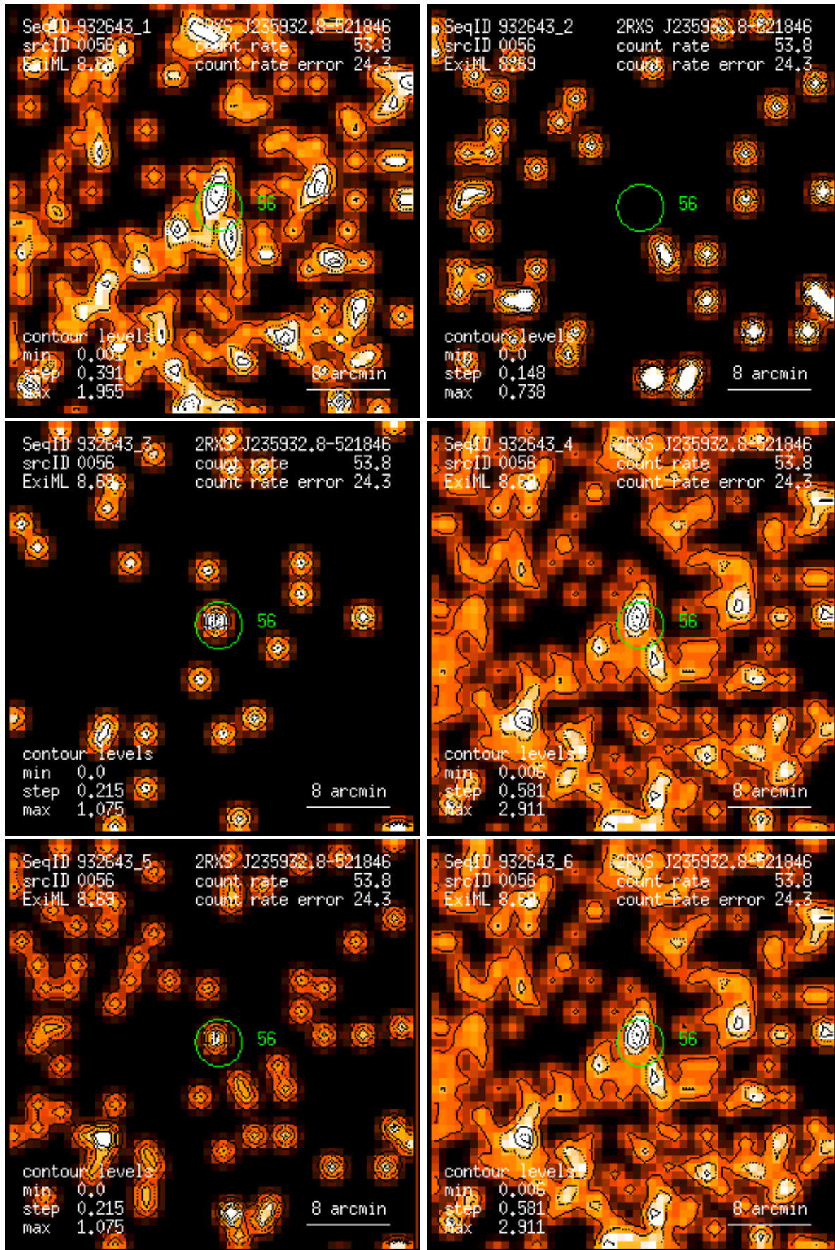
Figure 56: RASS 932643: detection 0056: band rate images, Gaussian filter: (1) PSPC channels 11 – 41, (2) 52 – 90, (3) 91 – 201, (4) 11 – 235, (5) 52 – 201, (6) 11 – 201. Broad band rates in counts/ks. Band rate contour levels in counts/ks/arcmin 2 .
