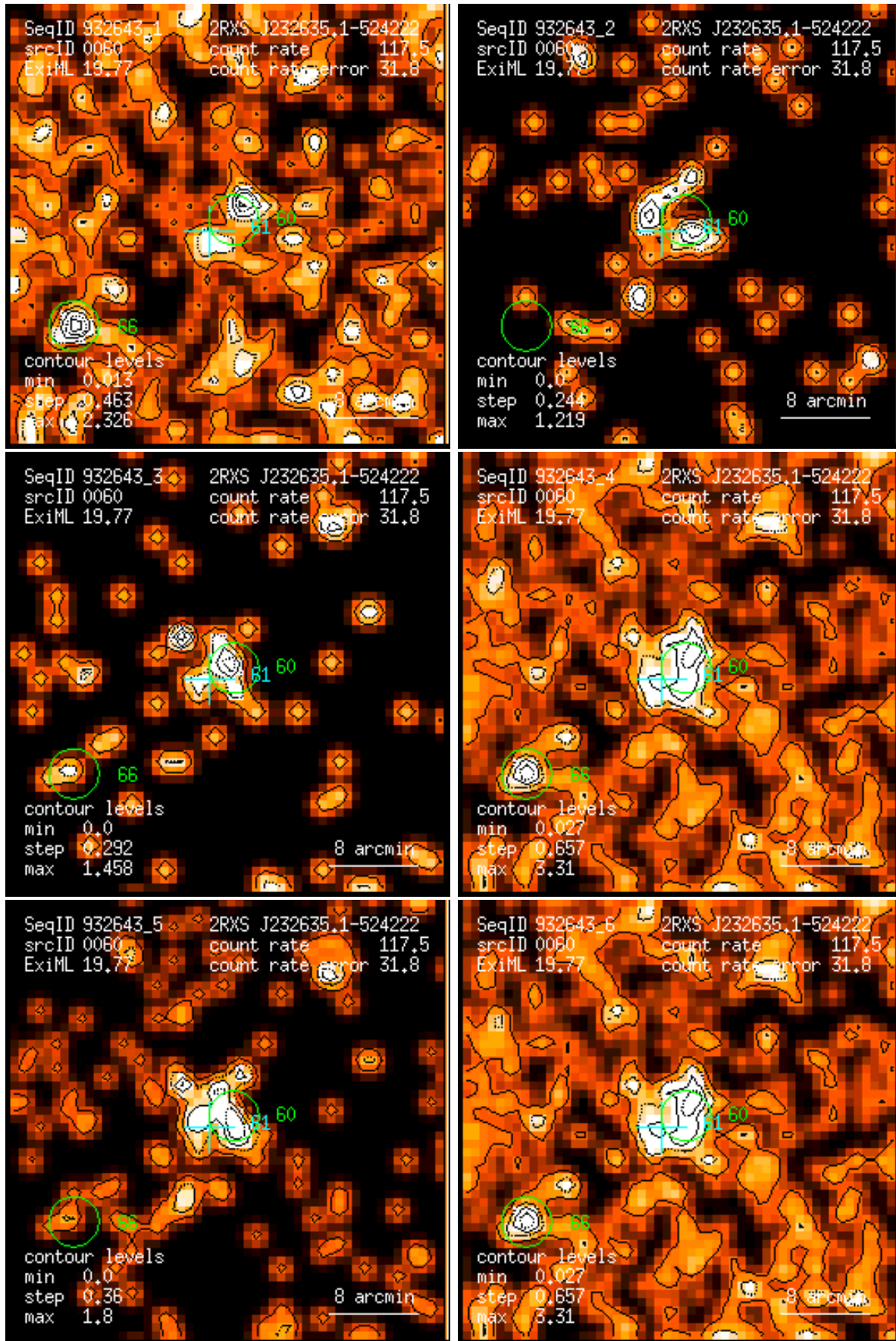
Figure 60: RASS 932643: detection 0060: band rate images, Gaussian filter: (1) PSPC channels 11 – 41, (2) 52 – 90, (3) 91 – 201, (4) 11 – 235, (5) 52 – 201, (6) 11 – 201. Broad band rates in counts/ks. Band rate contour levels in counts/ks/arcmin 2 .
