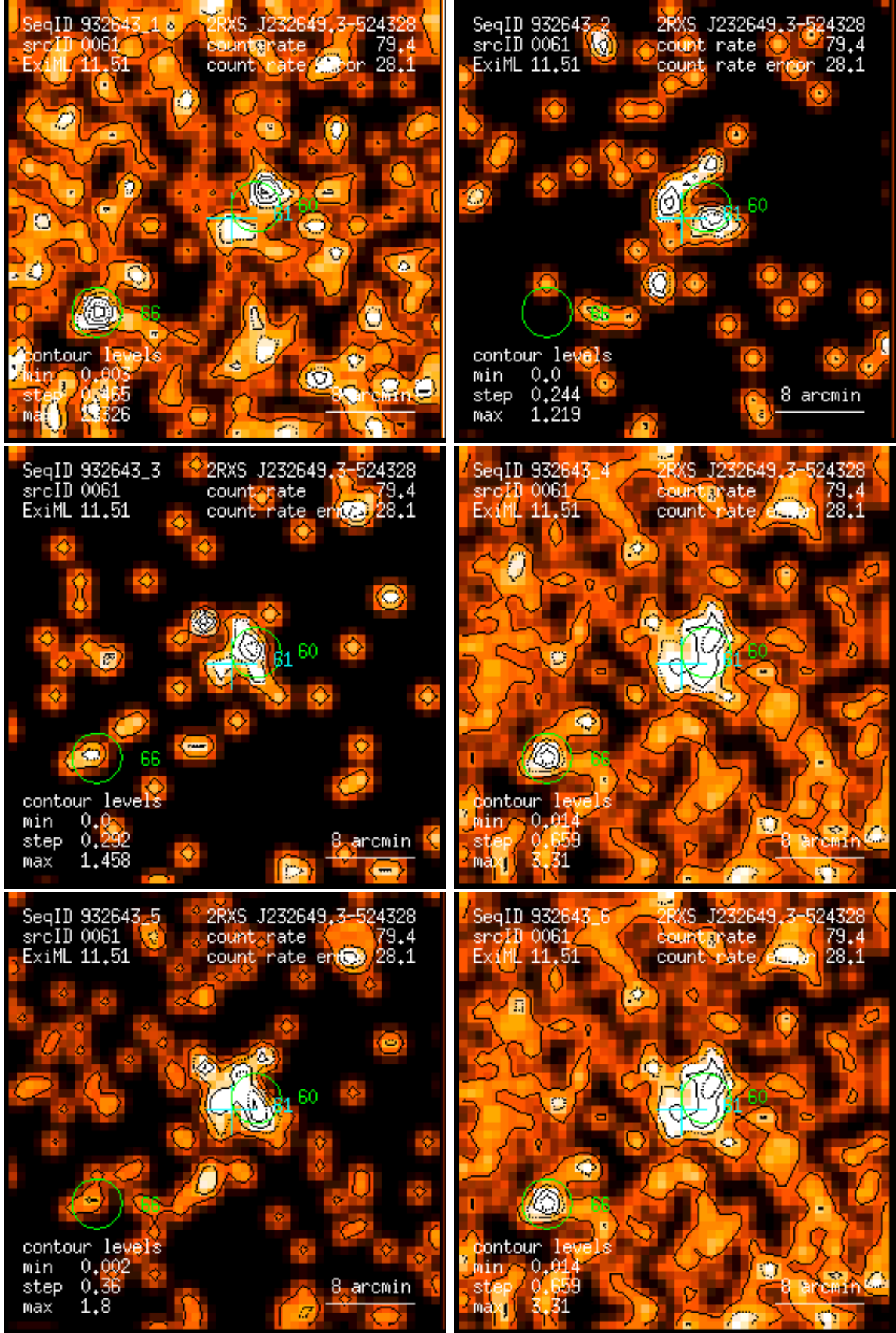
Figure 61: RASS 932643: detection 0061: band rate images, Gaussian filter: (1) PSPC channels 11 – 41, (2) 52 – 90, (3) 91 – 201, (4) 11 – 235, (5) 52 – 201, (6) 11 – 201. Broad band rates in counts/ks. Band rate contour levels in counts/ks/arcmin 2 .
