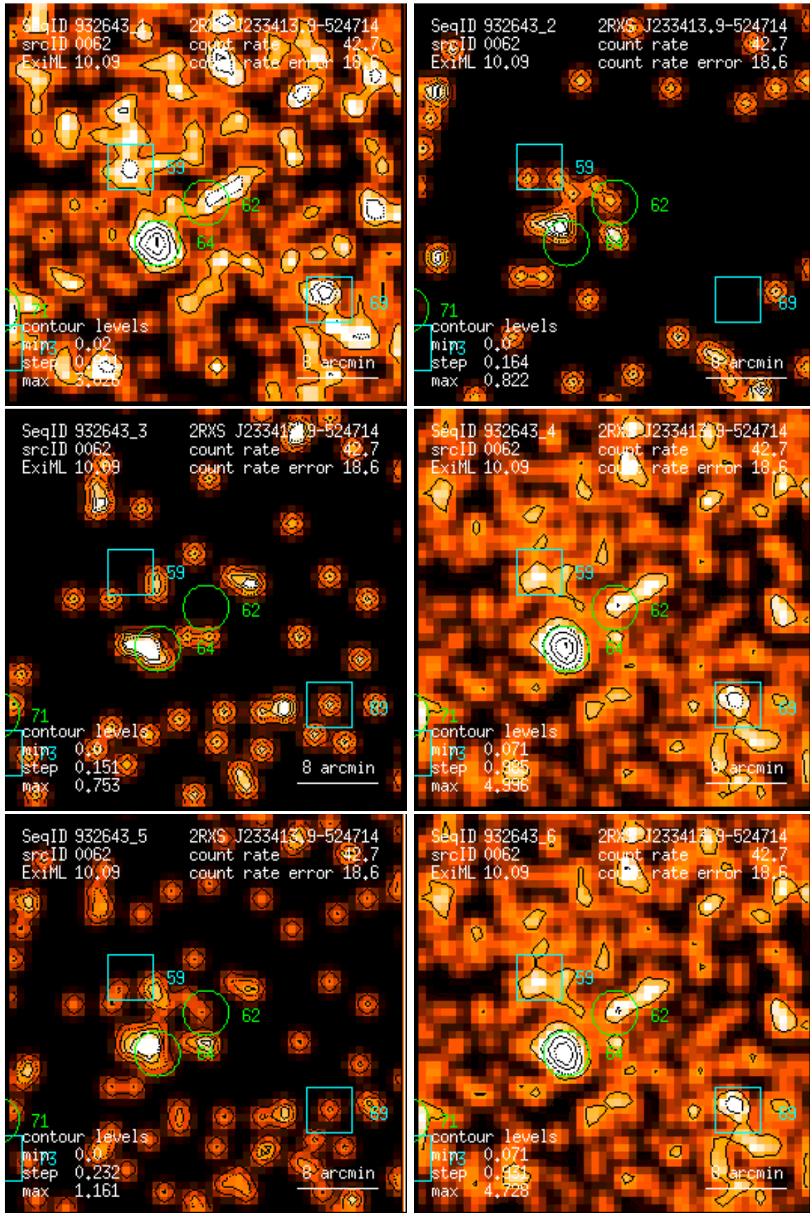
Figure 62: RASS 932643: detection 0062: band rate images, Gaussian filter: (1) PSPC channels 11 – 41, (2) 52 – 90, (3) 91 – 201, (4) 11 – 235, (5) 52 – 201, (6) 11 – 201. Broad band rates in counts/ks. Band rate contour levels in counts/ks/arcmin 2 .
