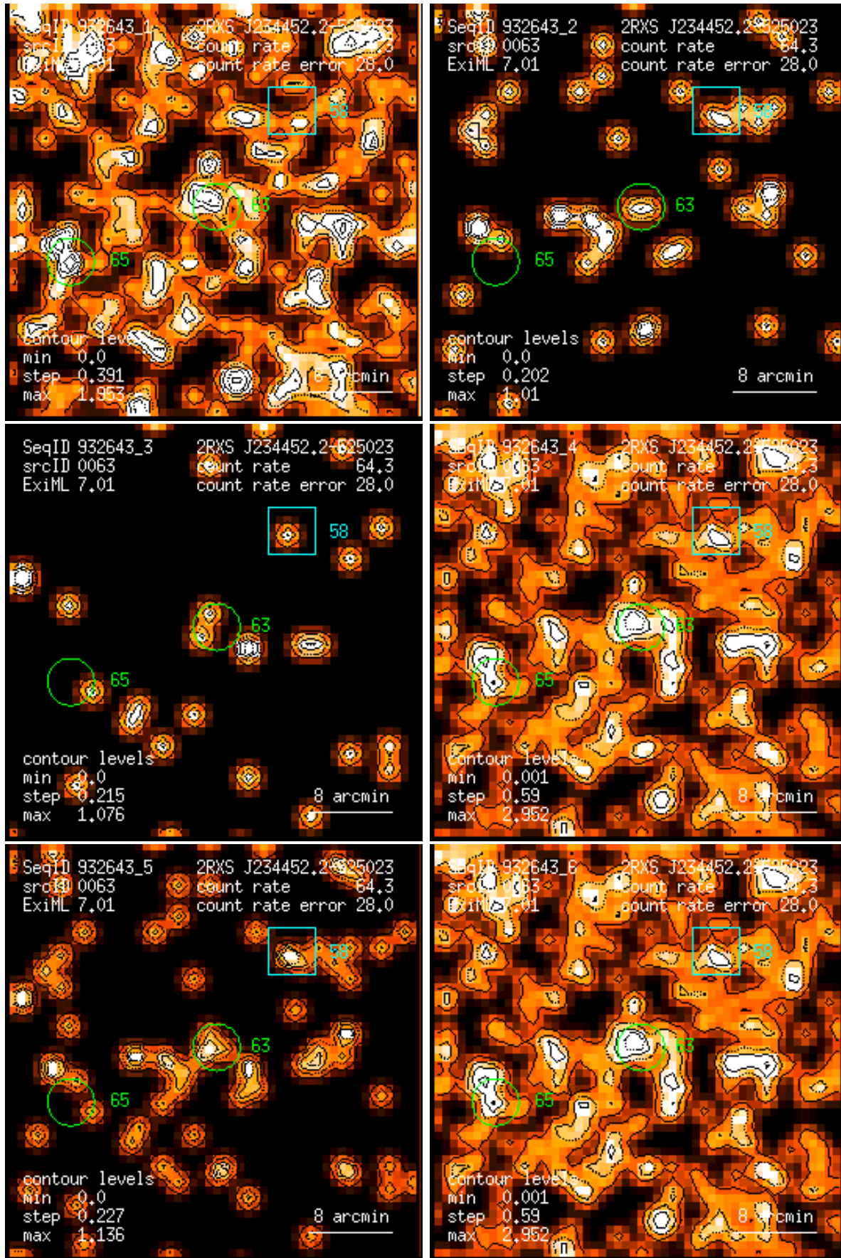
Figure 63: RASS 932643: detection 0063: band rate images, Gaussian filter: (1) PSPC channels 11 – 41, (2) 52 – 90, (3) 91 – 201, (4) 11 – 235, (5) 52 – 201, (6) 11 – 201. Broad band rates in counts/ks. Band rate contour levels in counts/ks/arcmin 2 .
