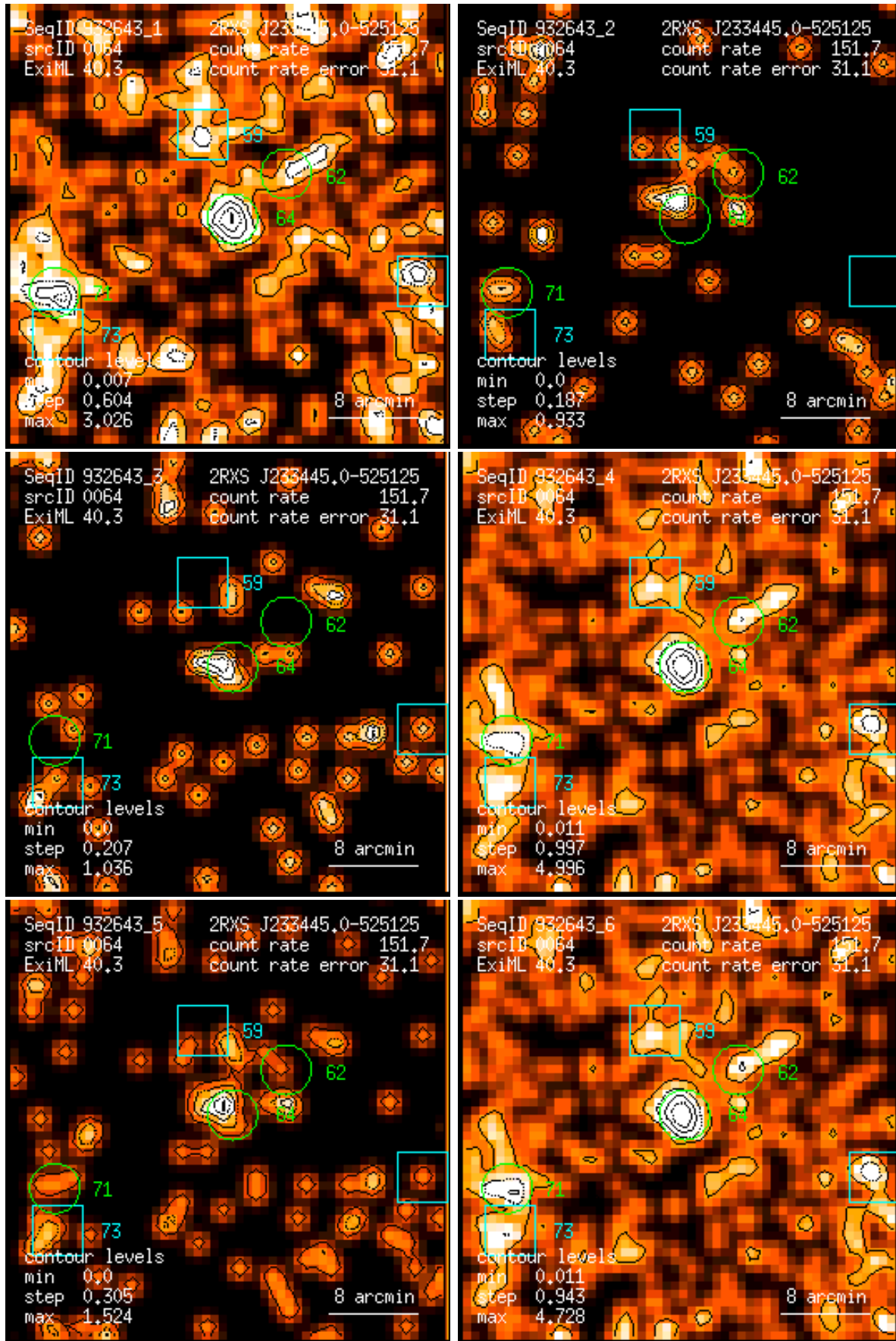
Figure 64: RASS 932643: detection 0064: band rate images, Gaussian filter: (1) PSPC channels 11 – 41, (2) 52 – 90, (3) 91 – 201, (4) 11 – 235, (5) 52 – 201, (6) 11 – 201. Broad band rates in counts/ks. Band rate contour levels in counts/ks/arcmin 2 .
