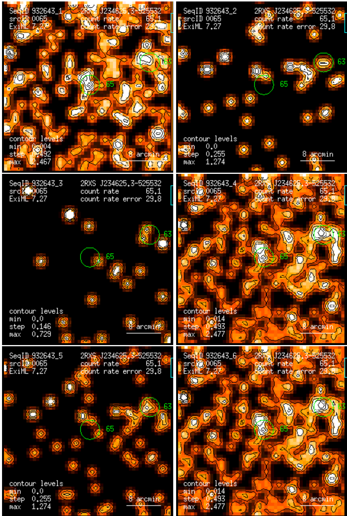
Figure 65: RASS 932643: detection 0065: band rate images, Gaussian filter: (1) PSPC channels 11 – 41, (2) 52 – 90, (3) 91 – 201, (4) 11 – 235, (5) 52 – 201, (6) 11 – 201. Broad band rates in counts/ks. Band rate contour levels in counts/ks/arcmin 2 .
