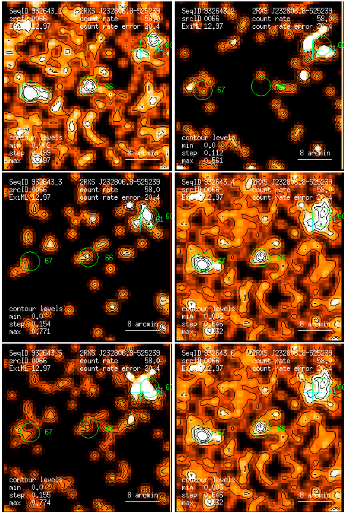
Figure 66: RASS 932643: detection 0066: band rate images, Gaussian filter: (1) PSPC channels 11 – 41, (2) 52 – 90, (3) 91 – 201, (4) 11 – 235, (5) 52 – 201, (6) 11 – 201. Broad band rates in counts/ks. Band rate contour levels in counts/ks/arcmin 2 .
