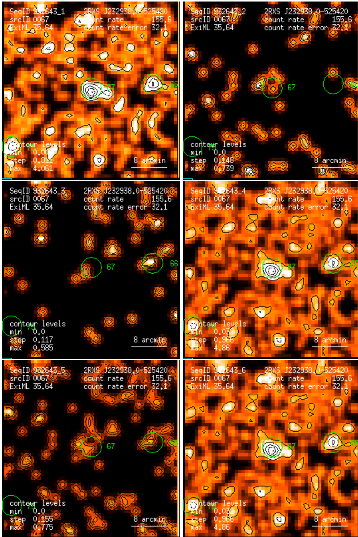
Figure 67: RASS 932643: detection 0067: band rate images, Gaussian filter: (1) PSPC channels 11 – 41, (2) 52 – 90, (3) 91 – 201, (4) 11 – 235, (5) 52 – 201, (6) 11 – 201. Broad band rates in counts/ks. Band rate contour levels in counts/ks/arcmin 2 .
