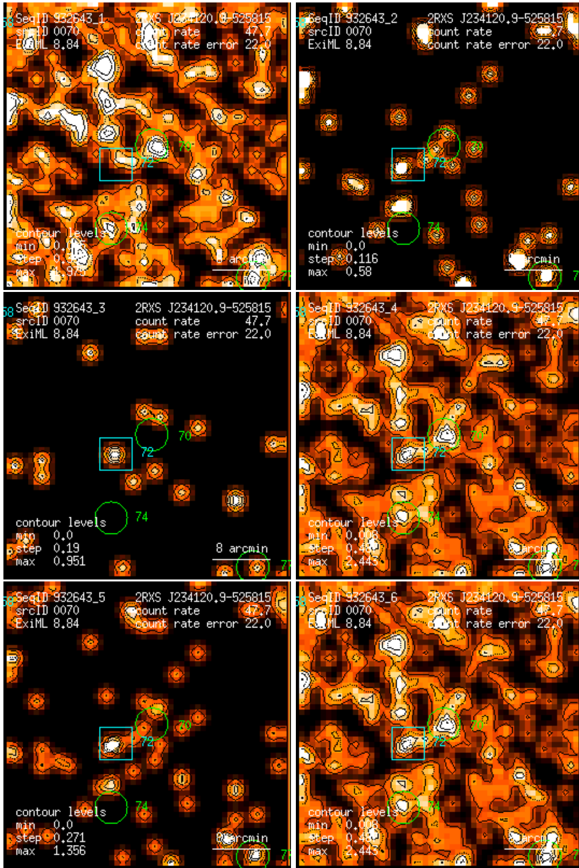
Figure 70: RASS 932643: detection 0070: band rate images, Gaussian filter: (1) PSPC channels 11 – 41, (2) 52 – 90, (3) 91 – 201, (4) 11 – 235, (5) 52 – 201, (6) 11 – 201. Broad band rates in counts/ks. Band rate contour levels in counts/ks/arcmin 2 .
