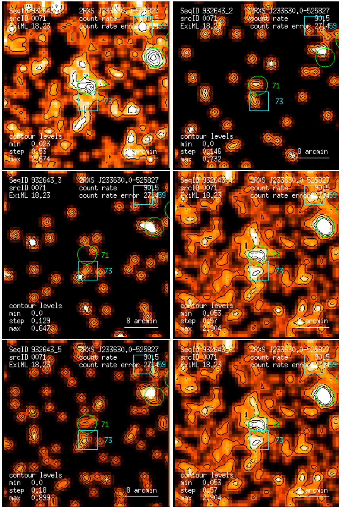
Figure 71: RASS 932643: detection 0071: band rate images, Gaussian filter: (1) PSPC channels 11 – 41, (2) 52 – 90, (3) 91 – 201, (4) 11 – 235, (5) 52 – 201, (6) 11 – 201. Broad band rates in counts/ks. Band rate contour levels in counts/ks/arcmin 2 .
