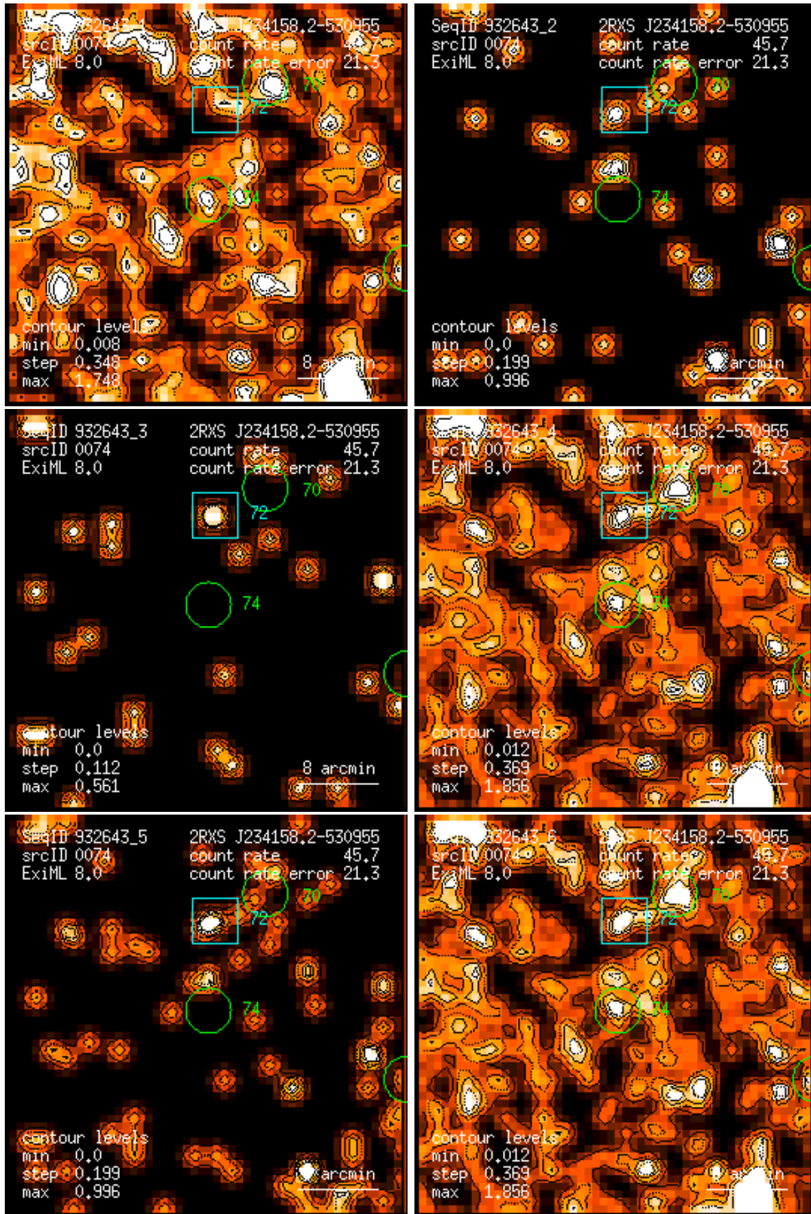
Figure 74: RASS 932643: detection 0074: band rate images, Gaussian filter: (1) PSPC channels 11 – 41, (2) 52 – 90, (3) 91 – 201, (4) 11 – 235, (5) 52 – 201, (6) 11 – 201. Broad band rates in counts/ks. Band rate contour levels in counts/ks/arcmin 2 .
