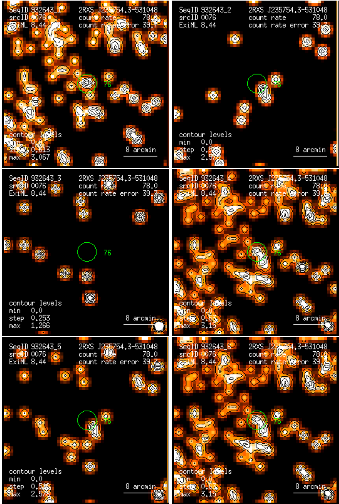
Figure 76: RASS 932643: detection 0076: band rate images, Gaussian filter: (1) PSPC channels 11 – 41, (2) 52 – 90, (3) 91 – 201, (4) 11 – 235, (5) 52 – 201, (6) 11 – 201. Broad band rates in counts/ks. Band rate contour levels in counts/ks/arcmin 2 .
