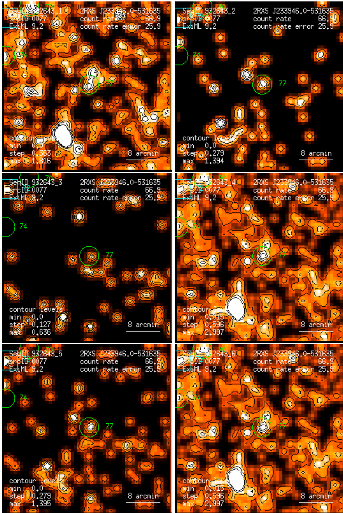
Figure 77: RASS 932643: detection 0077: band rate images, Gaussian filter: (1) PSPC channels 11 – 41, (2) 52 – 90, (3) 91 – 201, (4) 11 – 235, (5) 52 – 201, (6) 11 – 201. Broad band rates in counts/ks. Band rate contour levels in counts/ks/arcmin 2 .
