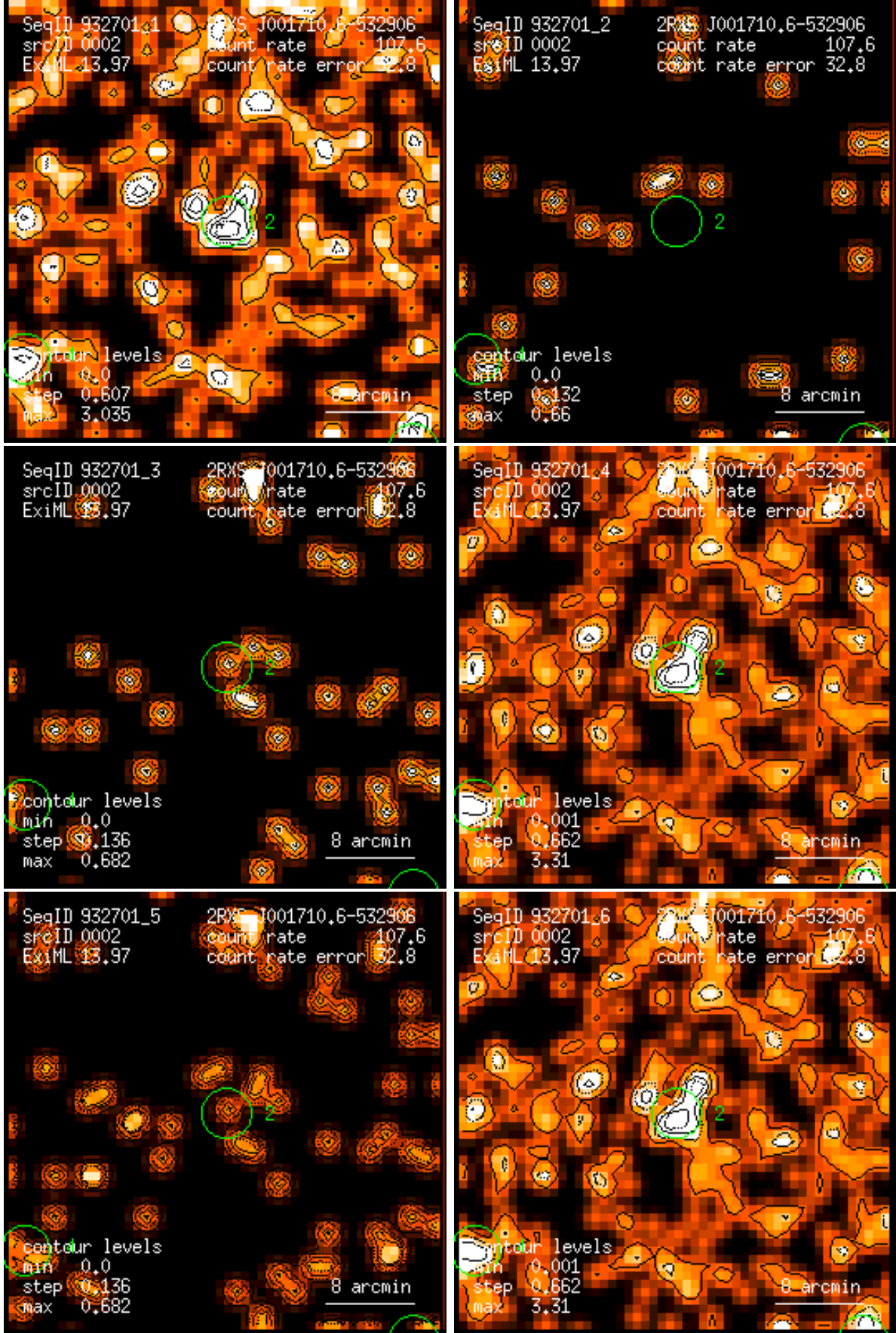
Figure 2: RASS 932701: detection 0002: band rate images, Gaussian filter: (1) PSPC channels 11 – 41, (2) 52 – 90, (3) 91 – 201, (4) 11 – 235, (5) 52 – 201, (6) 11 – 201. Broad band rates in counts/ks. Band rate contour levels in counts/ks/arcmin 2 .
