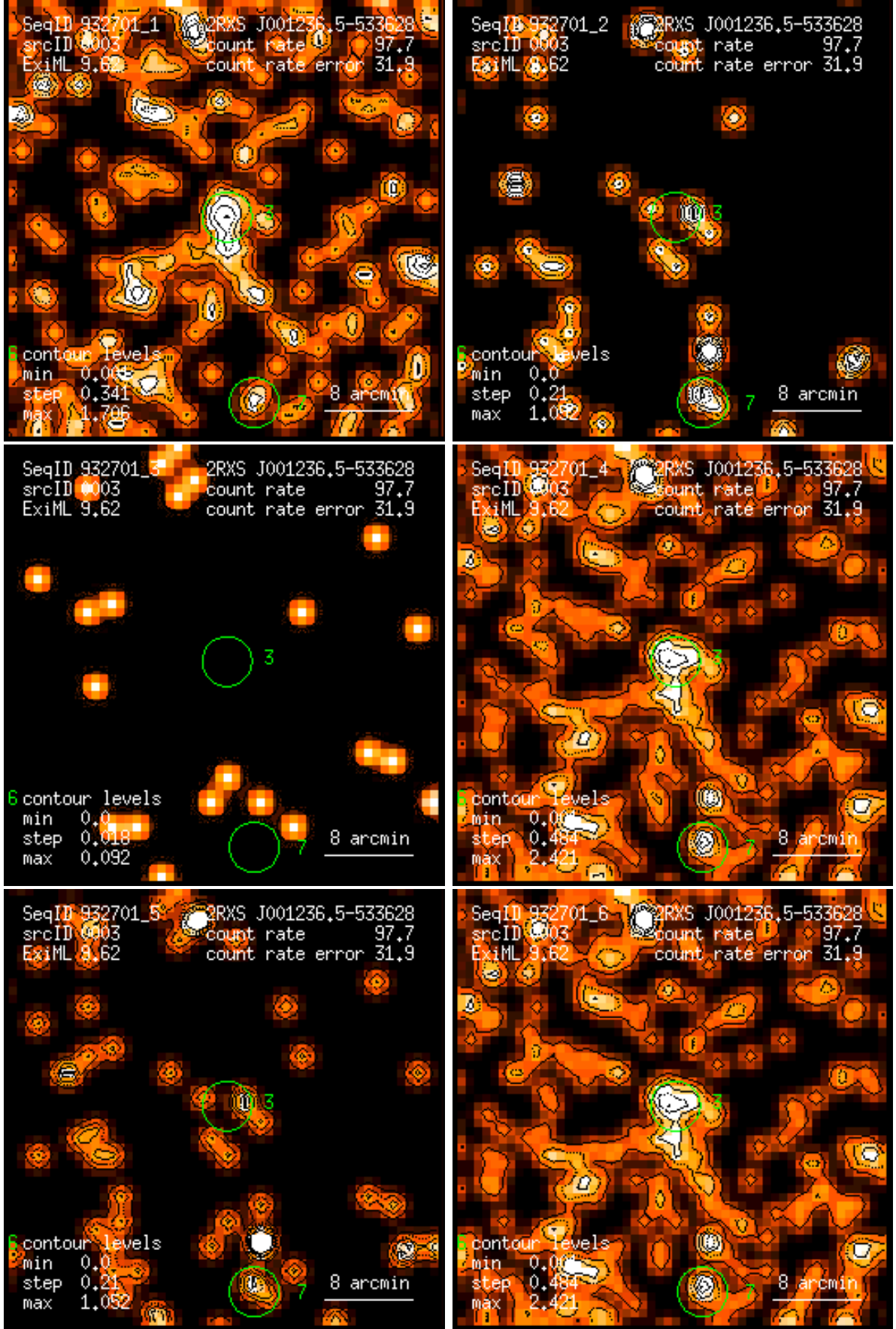
Figure 3: RASS 932701: detection 0003: band rate images, Gaussian filter: (1) PSPC channels 11 – 41, (2) 52 – 90, (3) 91 – 201, (4) 11 – 235, (5) 52 – 201, (6) 11 – 201. Broad band rates in counts/ks. Band rate contour levels in counts/ks/arcmin 2 .
