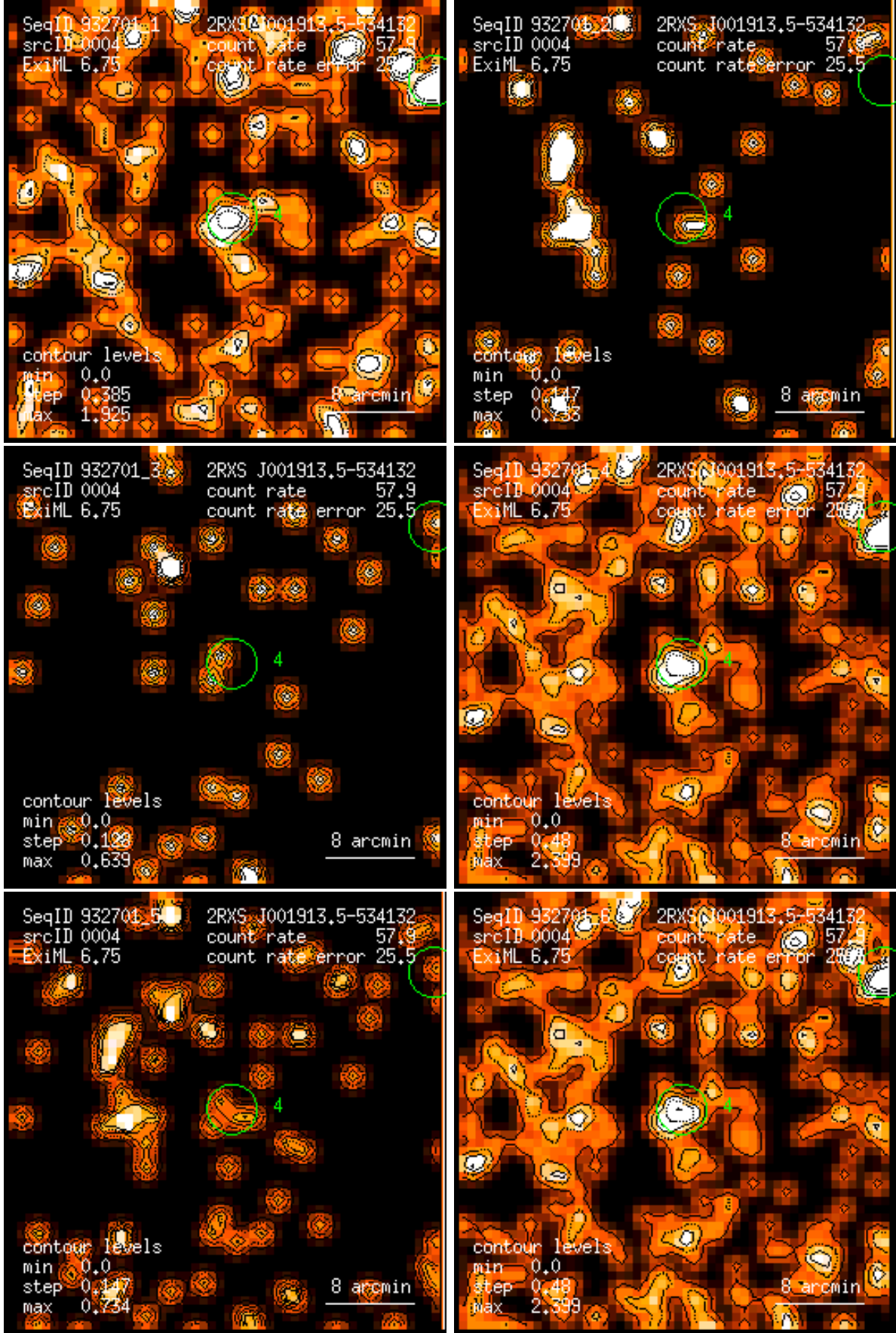
Figure 4: RASS 932701: detection 0004: band rate images, Gaussian filter: (1) PSPC channels 11 – 41, (2) 52 – 90, (3) 91 – 201, (4) 11 – 235, (5) 52 – 201, (6) 11 – 201. Broad band rates in counts/ks. Band rate contour levels in counts/ks/arcmin 2 .
