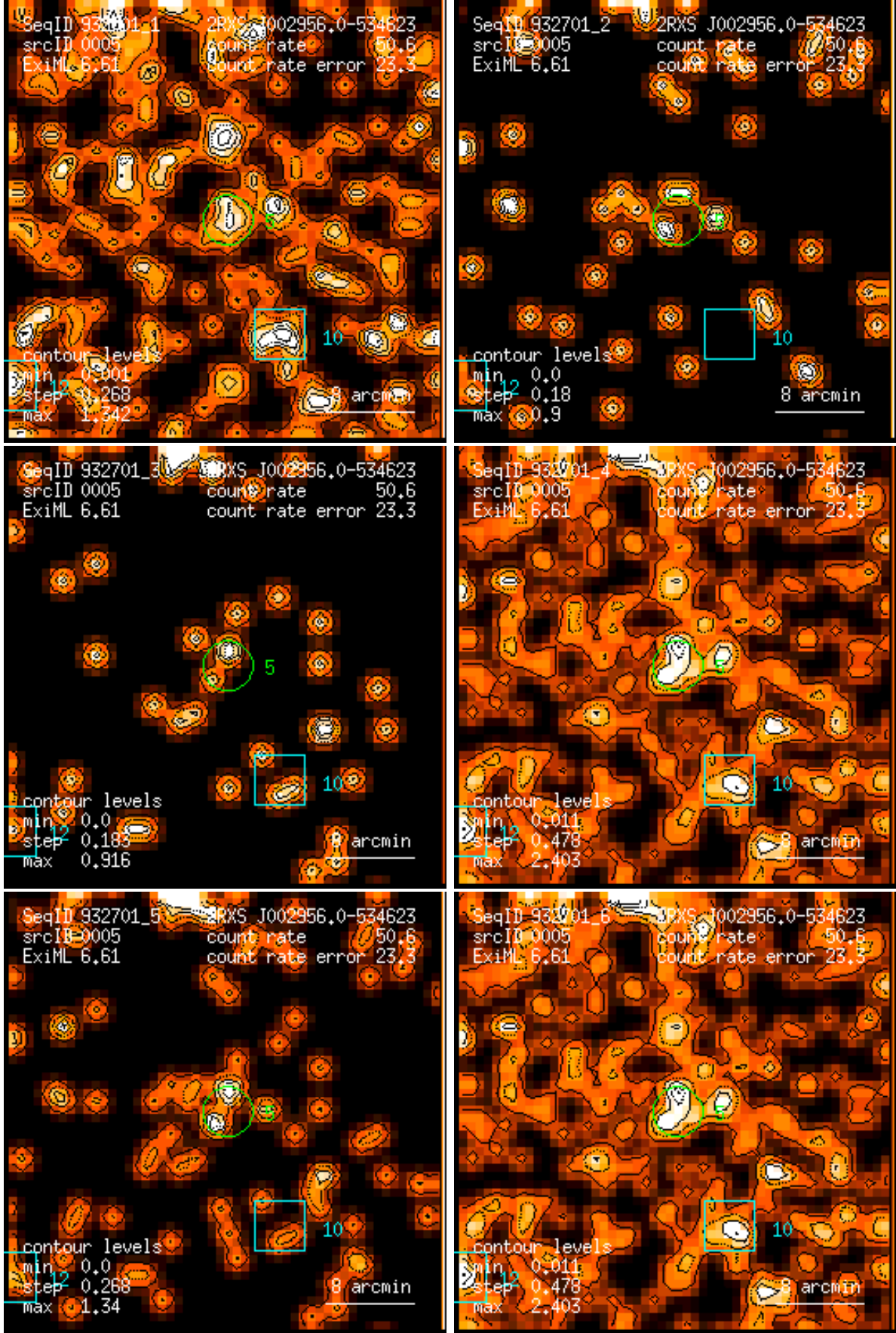
Figure 5: RASS 932701: detection 0005: band rate images, Gaussian filter: (1) PSPC channels 11 – 41, (2) 52 – 90, (3) 91 – 201, (4) 11 – 235, (5) 52 – 201, (6) 11 – 201. Broad band rates in counts/ks. Band rate contour levels in counts/ks/arcmin 2 .
