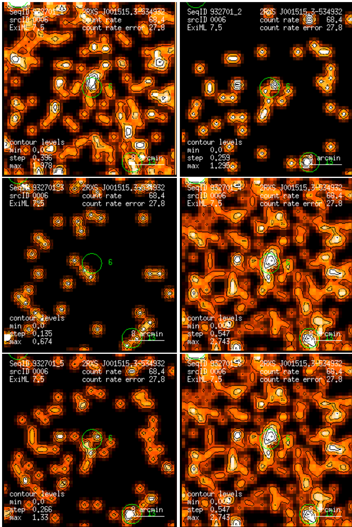
Figure 6: RASS 932701: detection 0006: band rate images, Gaussian filter: (1) PSPC channels 11 – 41, (2) 52 – 90, (3) 91 – 201, (4) 11 – 235, (5) 52 – 201, (6) 11 – 201. Broad band rates in counts/ks. Band rate contour levels in counts/ks/arcmin 2 .
