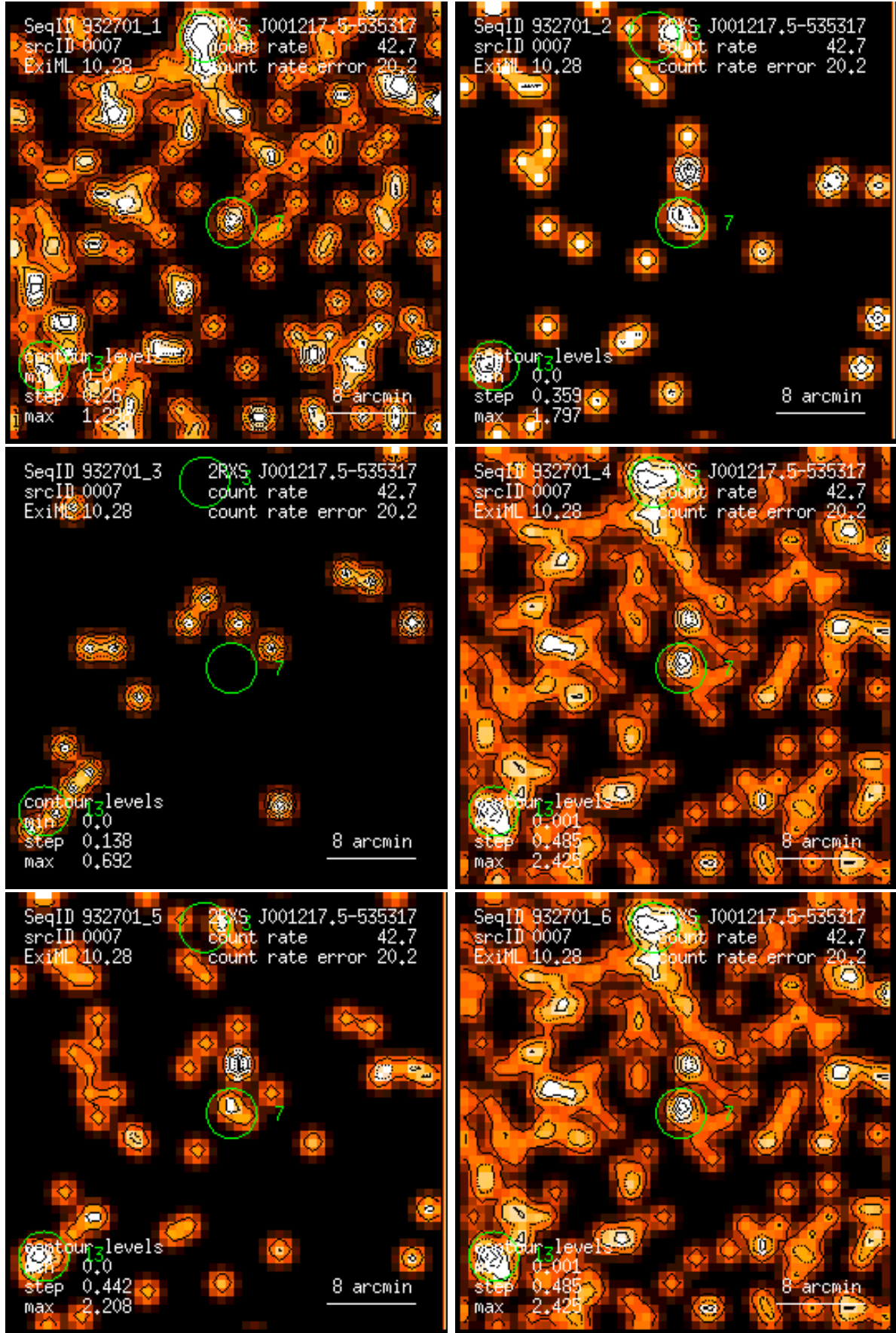
Figure 7: RASS 932701: detection 0007: band rate images, Gaussian filter: (1) PSPC channels 11 – 41, (2) 52 – 90, (3) 91 – 201, (4) 11 – 235, (5) 52 – 201, (6) 11 – 201. Broad band rates in counts/ks. Band rate contour levels in counts/ks/arcmin 2 .
