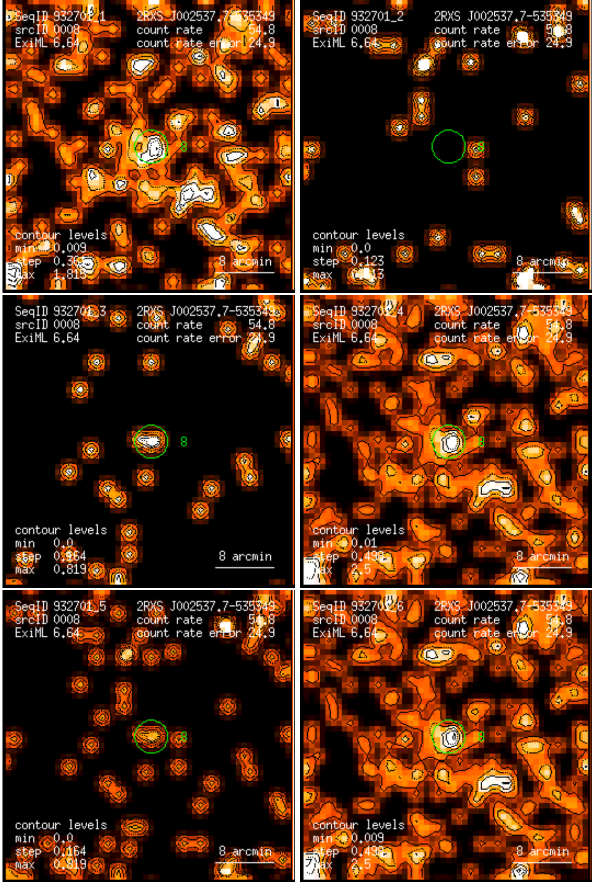
Figure 8: RASS 932701: detection 0008: band rate images, Gaussian filter: (1) PSPC channels 11 – 41, (2) 52 – 90, (3) 91 – 201, (4) 11 – 235, (5) 52 – 201, (6) 11 – 201. Broad band rates in counts/ks. Band rate contour levels in counts/ks/arcmin 2 .
