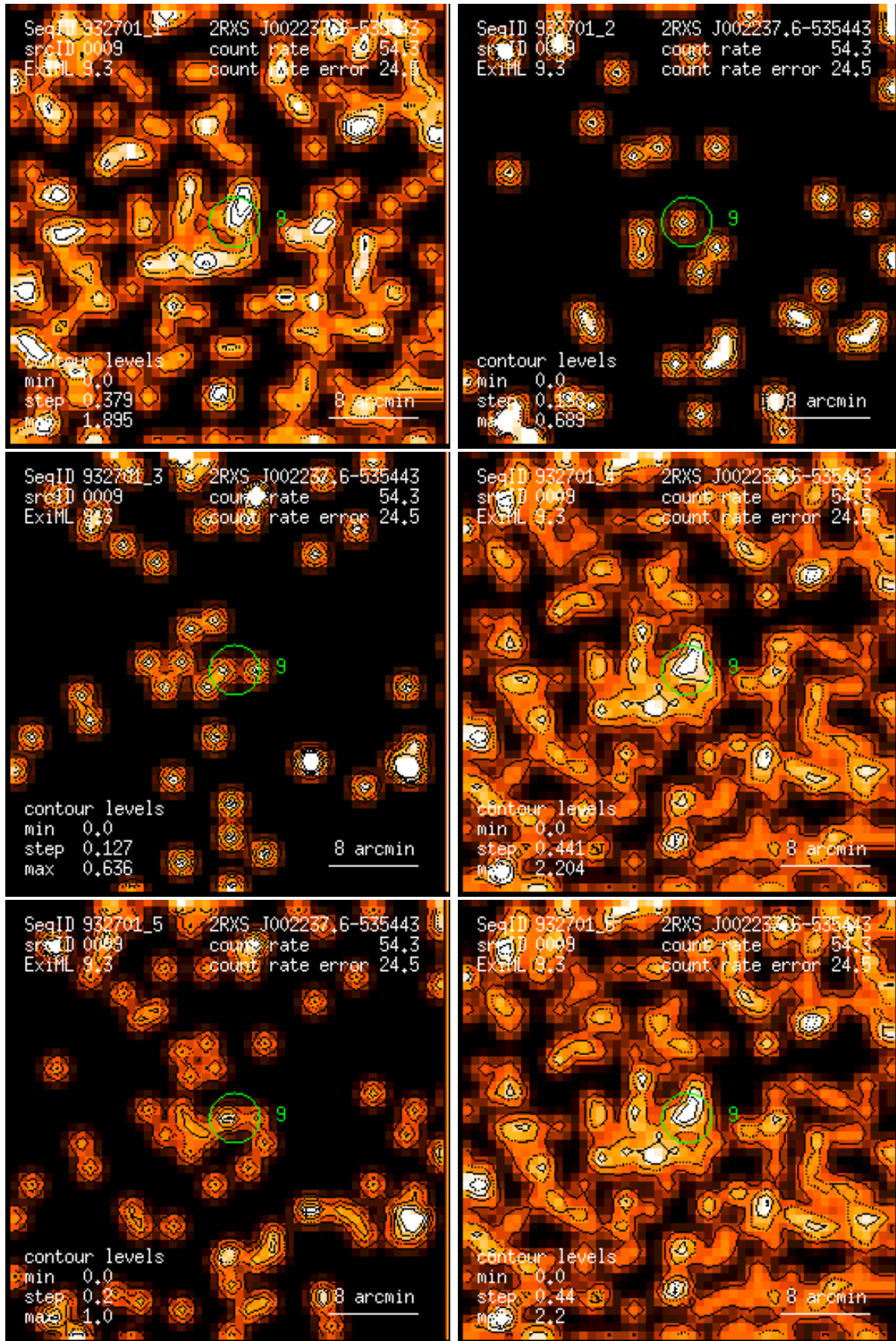
Figure 9: RASS 932701: detection 0009: band rate images, Gaussian filter: (1) PSPC channels 11 – 41, (2) 52 – 90, (3) 91 – 201, (4) 11 – 235, (5) 52 – 201, (6) 11 – 201. Broad band rates in counts/ks. Band rate contour levels in counts/ks/arcmin 2 .
