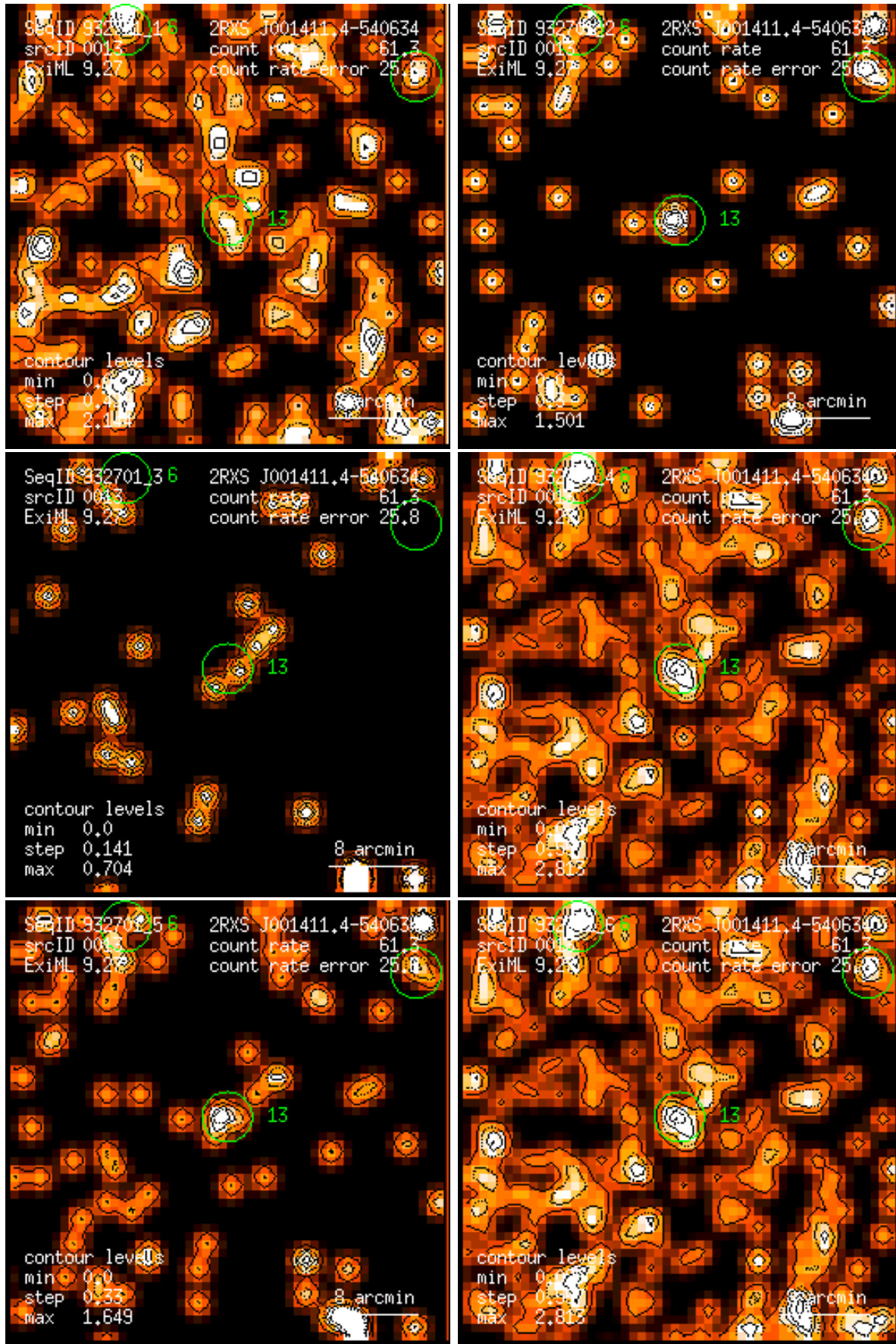
Figure 13: RASS 932701: detection 0013: band rate images, Gaussian filter: (1) PSPC channels 11 – 41, (2) 52 – 90, (3) 91 – 201, (4) 11 – 235, (5) 52 – 201, (6) 11 – 201. Broad band rates in counts/ks. Band rate contour levels in counts/ks/arcmin 2 .
