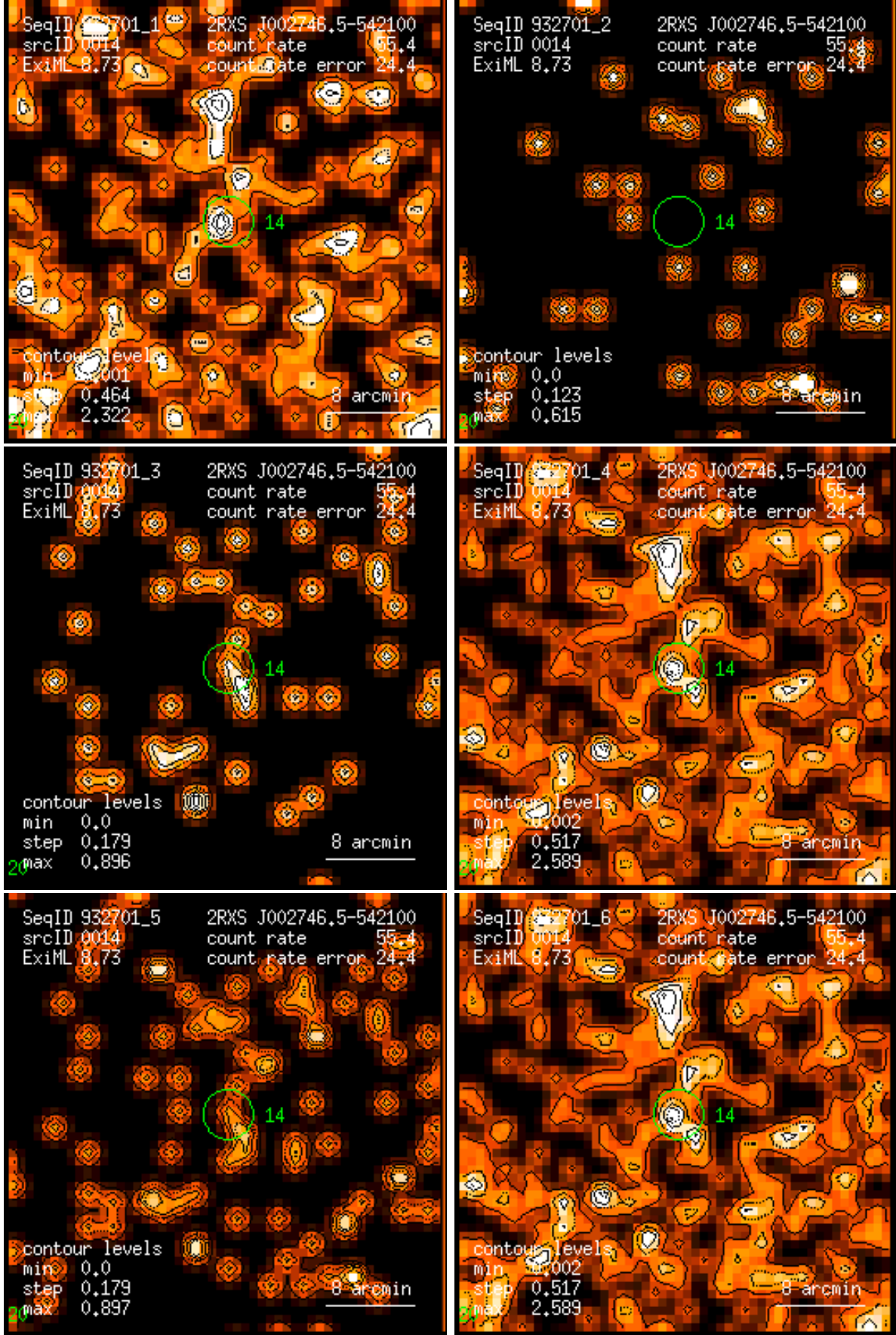
Figure 14: RASS 932701: detection 0014: band rate images, Gaussian filter: (1) PSPC channels 11 – 41, (2) 52 – 90, (3) 91 – 201, (4) 11 – 235, (5) 52 – 201, (6) 11 – 201. Broad band rates in counts/ks. Band rate contour levels in counts/ks/arcmin 2 .
