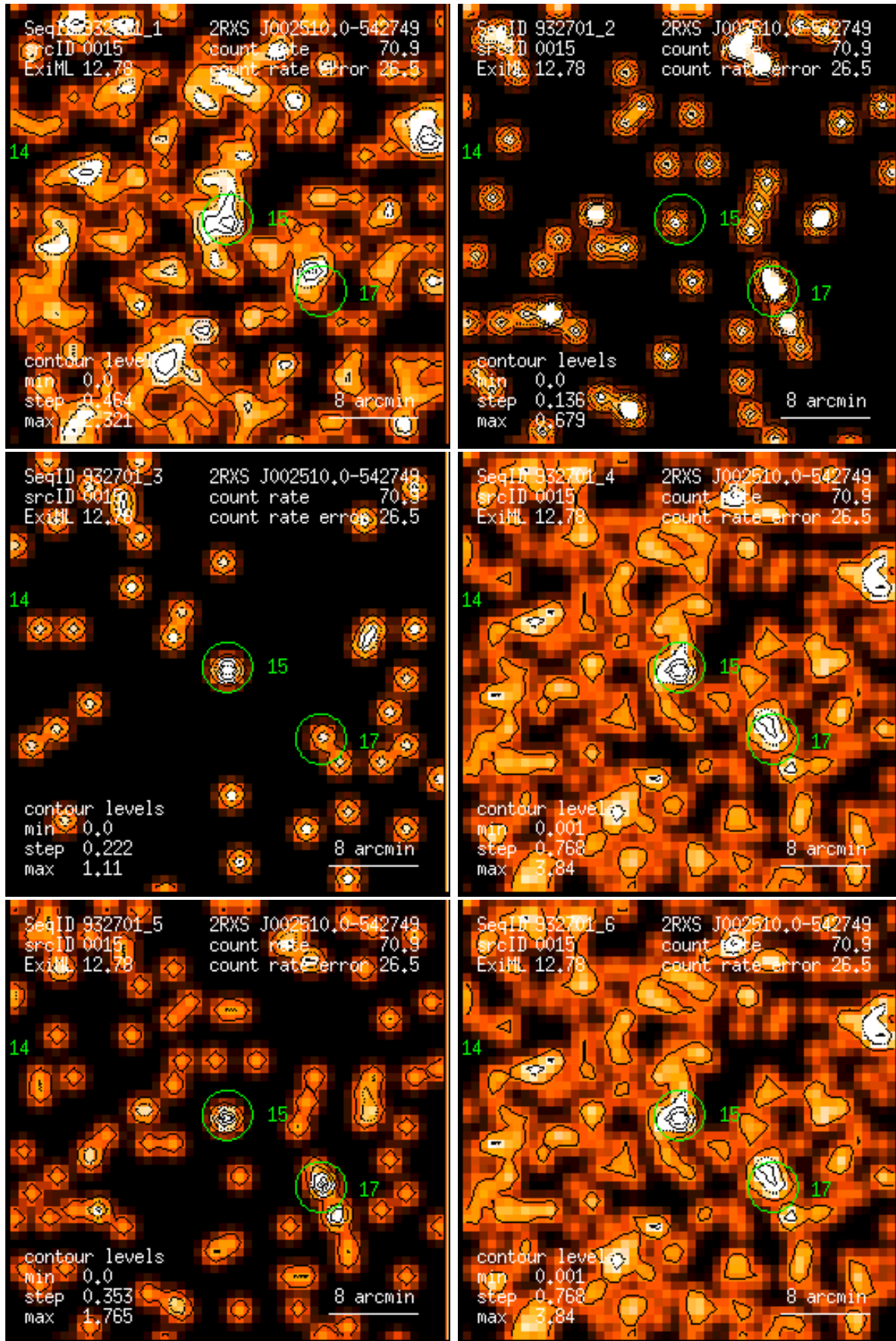
Figure 15: RASS 932701: detection 0015: band rate images, Gaussian filter: (1) PSPC channels 11 – 41, (2) 52 – 90, (3) 91 – 201, (4) 11 – 235, (5) 52 – 201, (6) 11 – 201. Broad band rates in counts/ks. Band rate contour levels in counts/ks/arcmin 2 .
