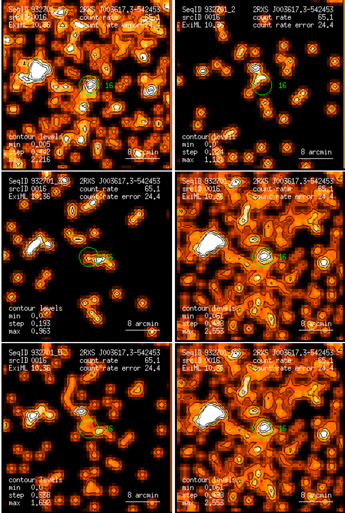
Figure 16: RASS 932701: detection 0016: band rate images, Gaussian filter: (1) PSPC channels 11 – 41, (2) 52 – 90, (3) 91 – 201, (4) 11 – 235, (5) 52 – 201, (6) 11 – 201. Broad band rates in counts/ks. Band rate contour levels in counts/ks/arcmin 2 .
