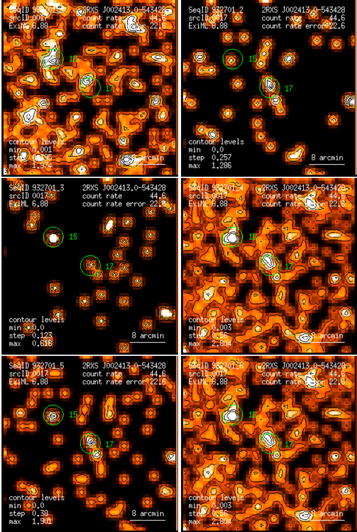
Figure 17: RASS 932701: detection 0017: band rate images, Gaussian filter: (1) PSPC channels 11 – 41, (2) 52 – 90, (3) 91 – 201, (4) 11 – 235, (5) 52 – 201, (6) 11 – 201. Broad band rates in counts/ks. Band rate contour levels in counts/ks/arcmin 2 .
