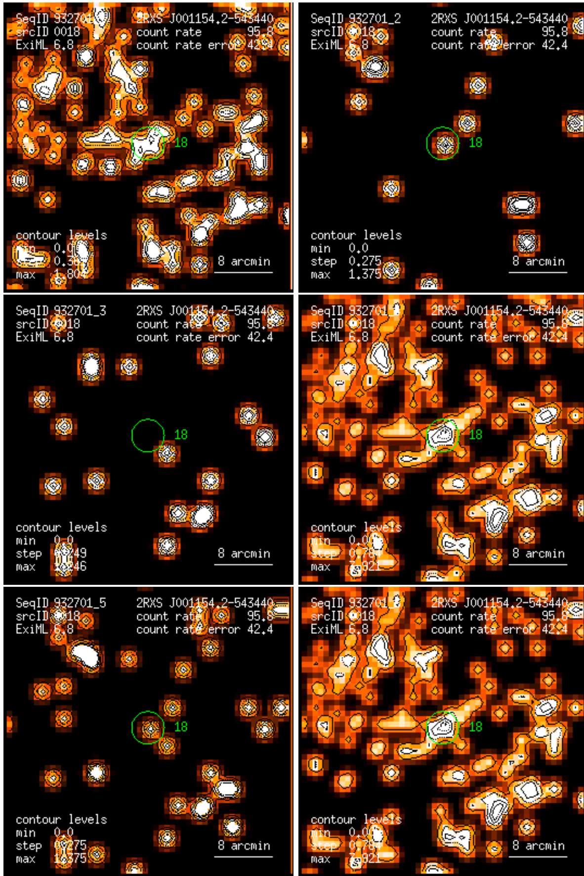
Figure 18: RASS 932701: detection 0018: band rate images, Gaussian filter: (1) PSPC channels 11 – 41, (2) 52 – 90, (3) 91 – 201, (4) 11 – 235, (5) 52 – 201, (6) 11 – 201. Broad band rates in counts/ks. Band rate contour levels in counts/ks/arcmin 2 .
