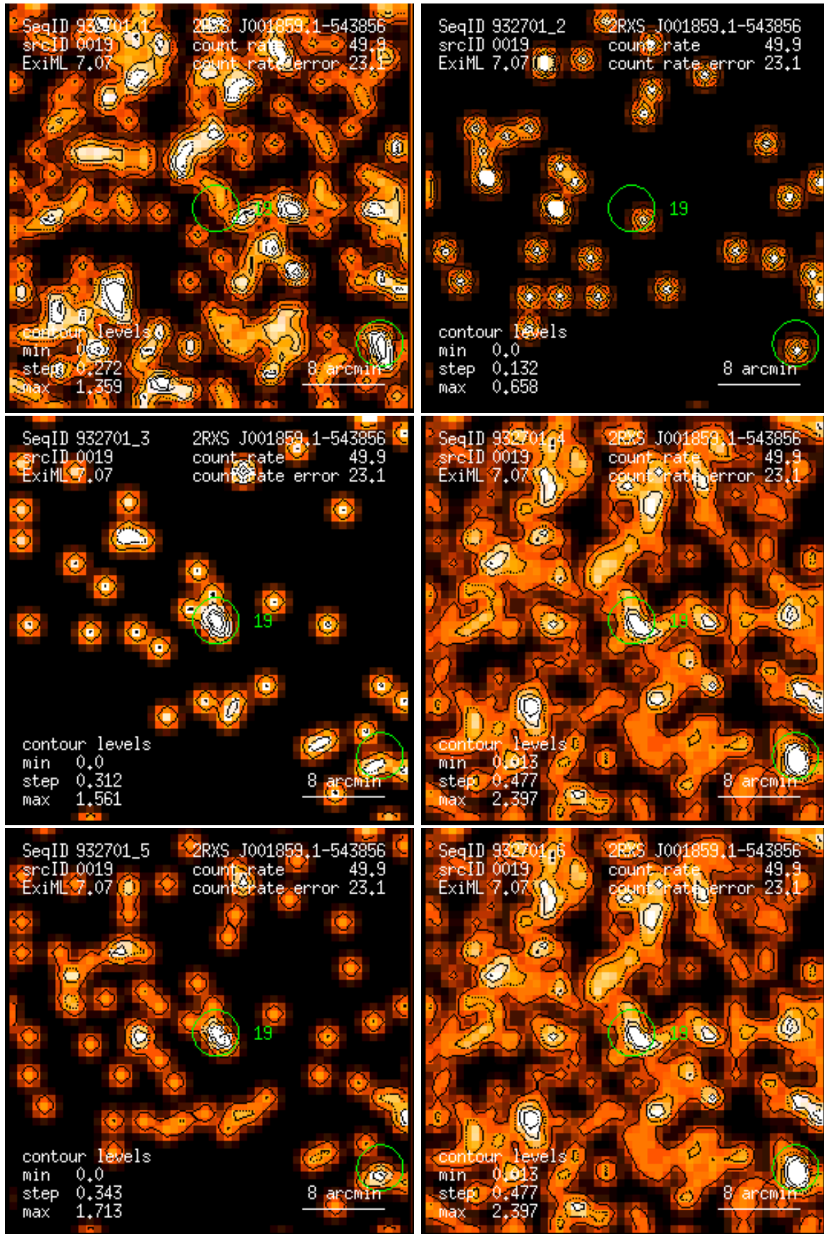
Figure 19: RASS 932701: detection 0019: band rate images, Gaussian filter: (1) PSPC channels 11 – 41, (2) 52 – 90, (3) 91 – 201, (4) 11 – 235, (5) 52 – 201, (6) 11 – 201. Broad band rates in counts/ks. Band rate contour levels in counts/ks/arcmin 2 .
