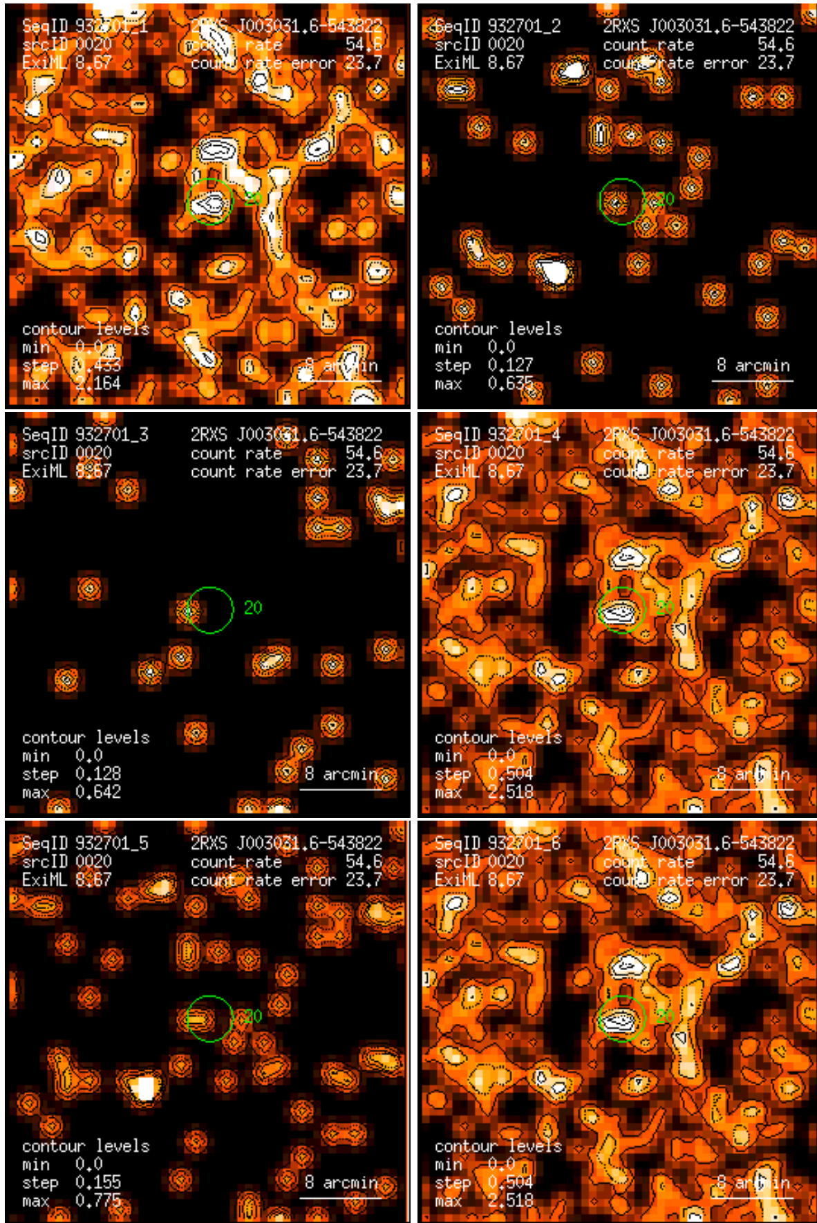
Figure 20: RASS 932701: detection 0020: band rate images, Gaussian filter: (1) PSPC channels 11 – 41, (2) 52 – 90, (3) 91 – 201, (4) 11 – 235, (5) 52 – 201, (6) 11 – 201. Broad band rates in counts/ks. Band rate contour levels in counts/ks/arcmin 2 .
