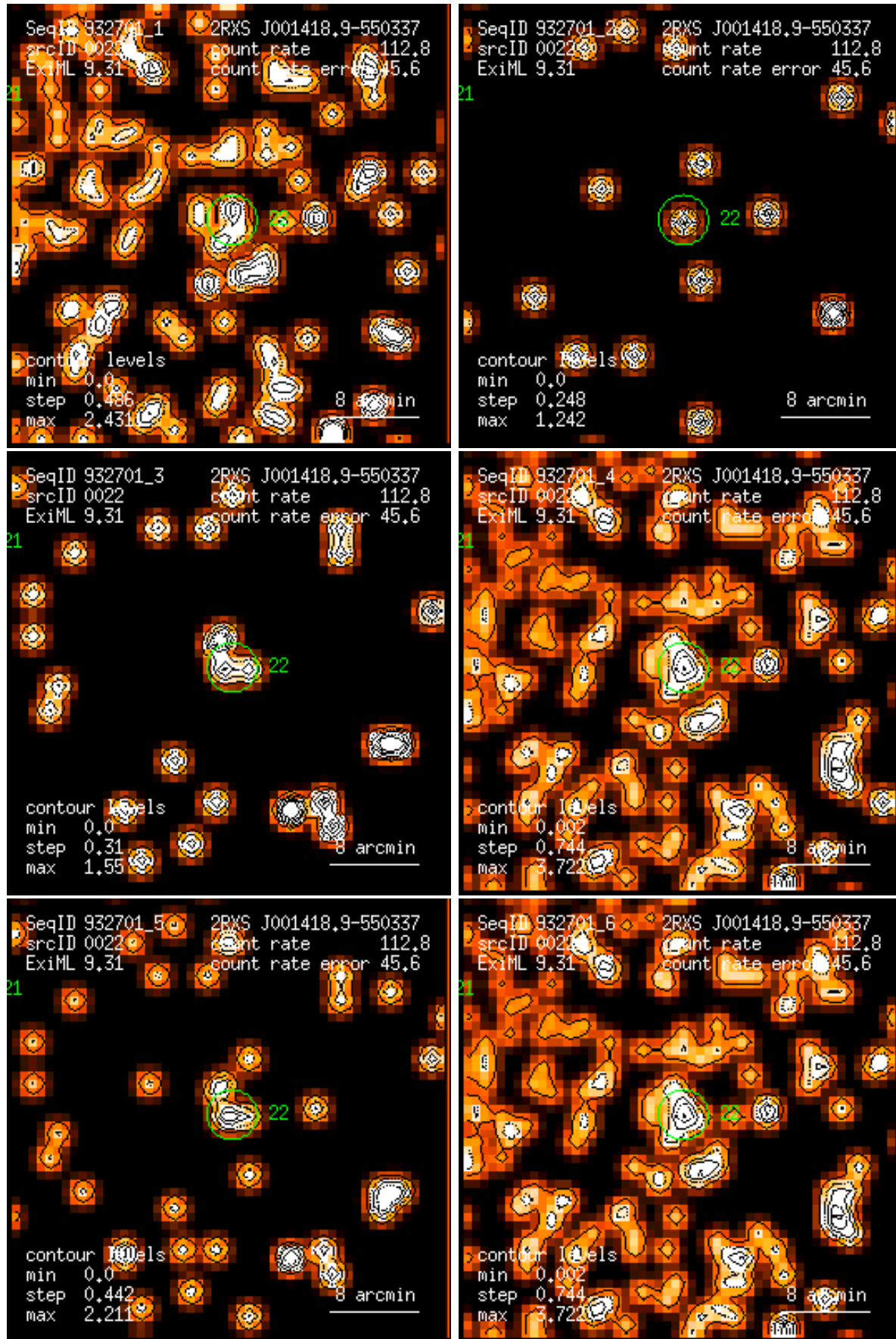
Figure 22: RASS 932701: detection 0022: band rate images, Gaussian filter: (1) PSPC channels 11 – 41, (2) 52 – 90, (3) 91 – 201, (4) 11 – 235, (5) 52 – 201, (6) 11 – 201. Broad band rates in counts/ks. Band rate contour levels in counts/ks/arcmin 2 .
