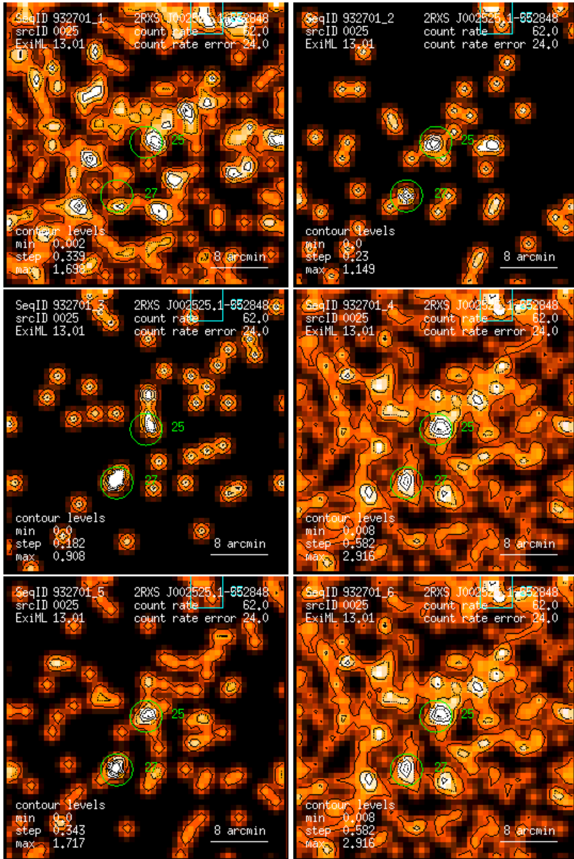
Figure 25: RASS 932701: detection 0025: band rate images, Gaussian filter: (1) PSPC channels 11 – 41, (2) 52 – 90, (3) 91 – 201, (4) 11 – 235, (5) 52 – 201, (6) 11 – 201. Broad band rates in counts/ks. Band rate contour levels in counts/ks/arcmin 2 .
