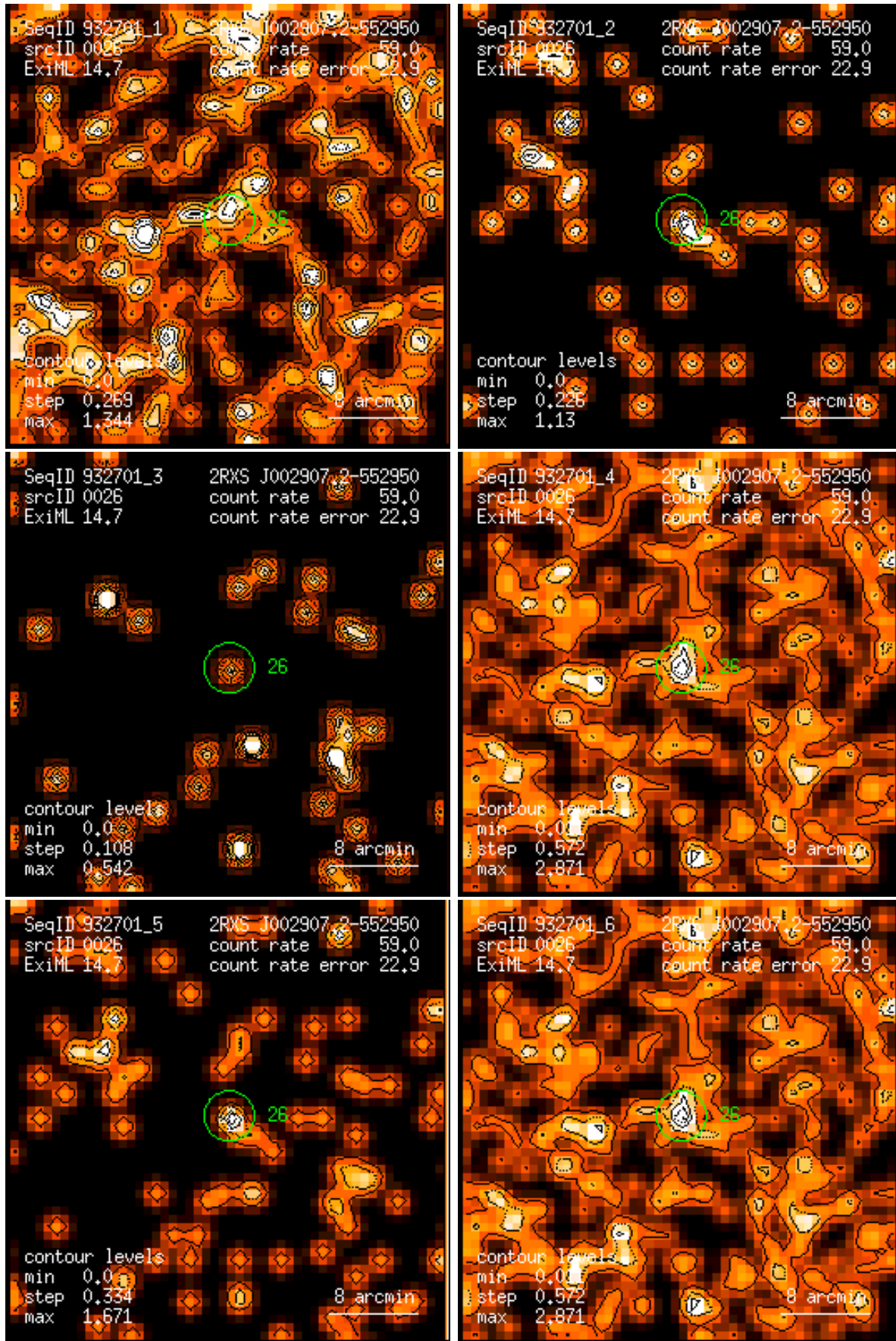
Figure 26: RASS 932701: detection 0026: band rate images, Gaussian filter: (1) PSPC channels 11 – 41, (2) 52 – 90, (3) 91 – 201, (4) 11 – 235, (5) 52 – 201, (6) 11 – 201. Broad band rates in counts/ks. Band rate contour levels in counts/ks/arcmin 2 .
