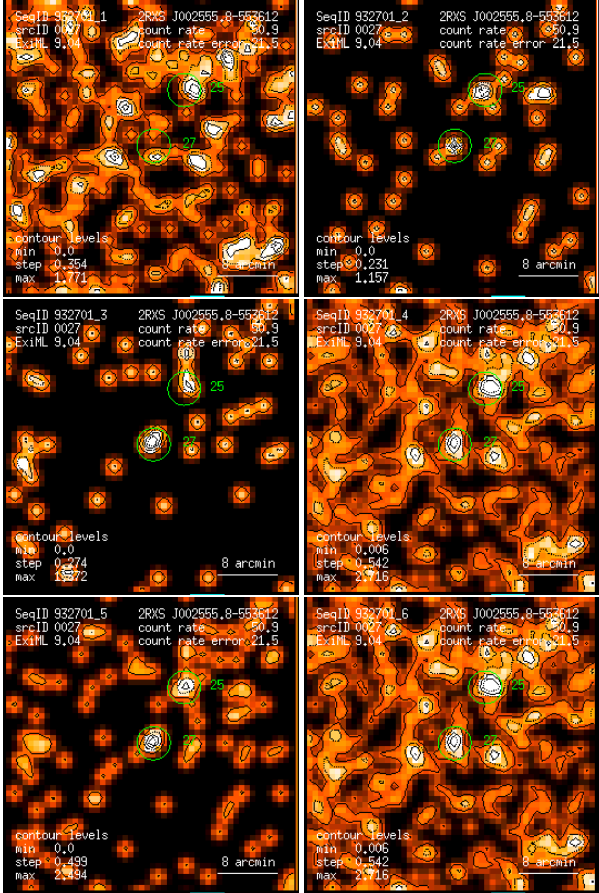
Figure 27: RASS 932701: detection 0027: band rate images, Gaussian filter: (1) PSPC channels 11 – 41, (2) 52 – 90, (3) 91 – 201, (4) 11 – 235, (5) 52 – 201, (6) 11 – 201. Broad band rates in counts/ks. Band rate contour levels in counts/ks/arcmin 2 .
