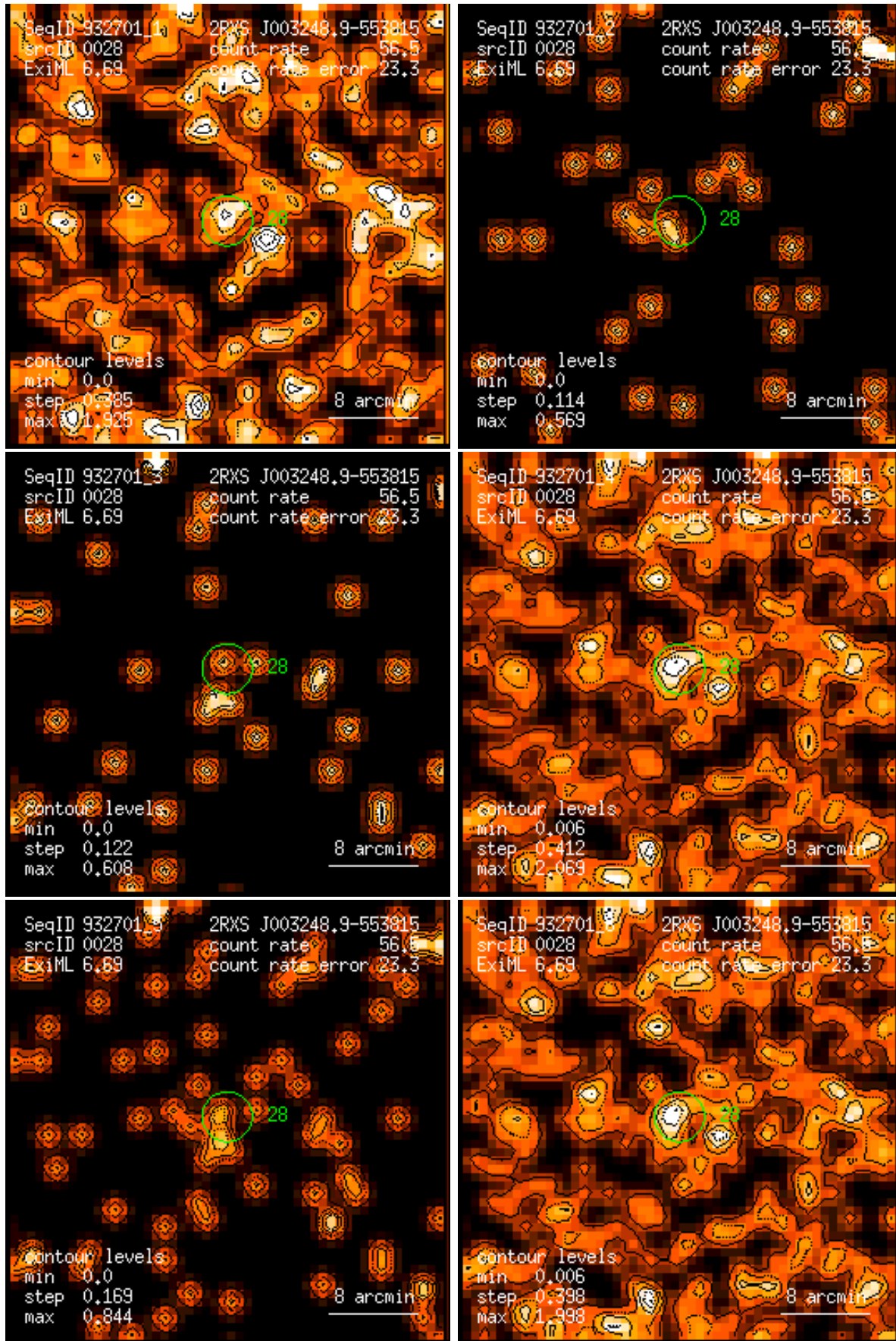
Figure 28: RASS 932701: detection 0028: band rate images, Gaussian filter: (1) PSPC channels 11 – 41, (2) 52 – 90, (3) 91 – 201, (4) 11 – 235, (5) 52 – 201, (6) 11 – 201. Broad band rates in counts/ks. Band rate contour levels in counts/ks/arcmin 2 .
