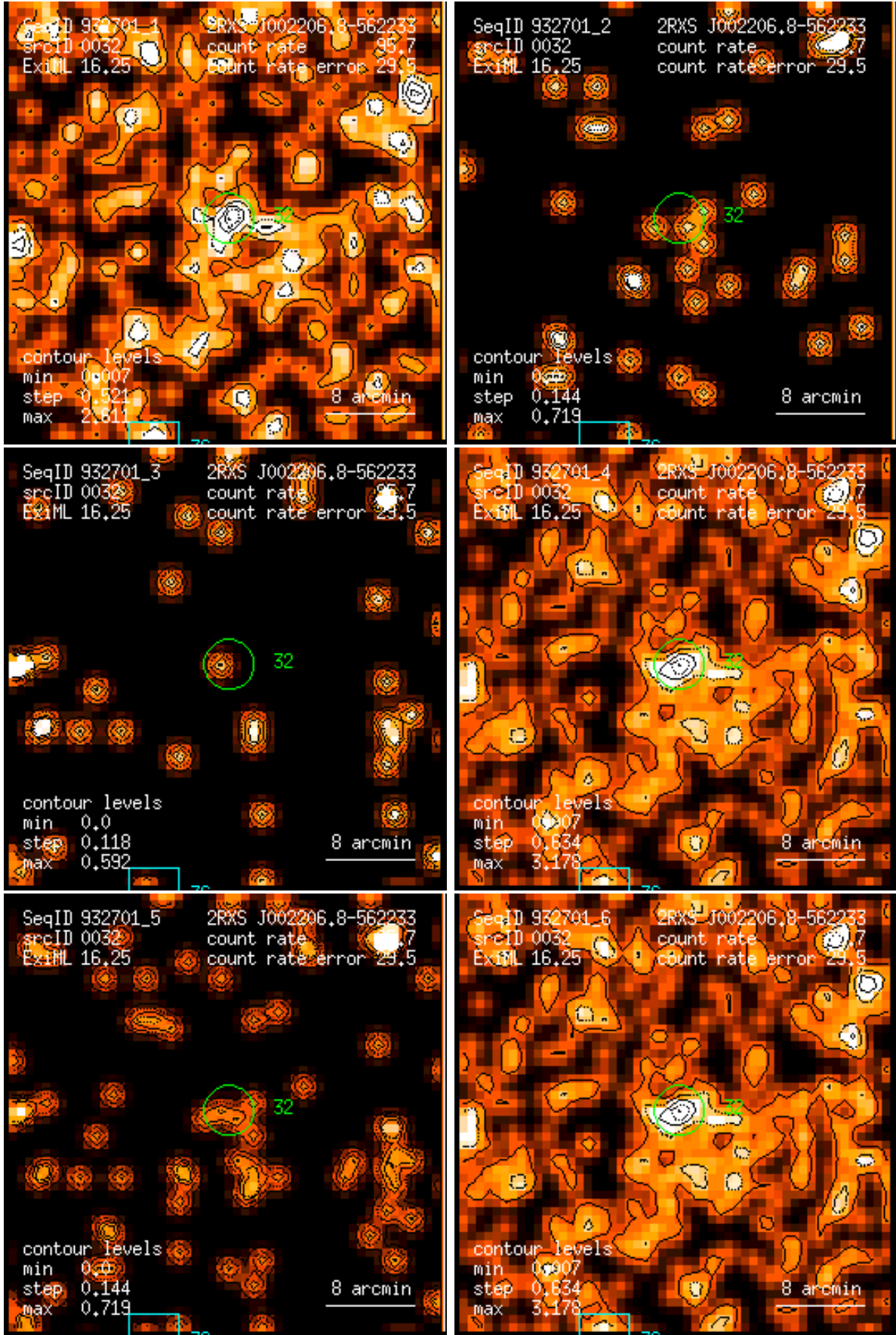
Figure 32: RASS 932701: detection 0032: band rate images, Gaussian filter: (1) PSPC channels 11 – 41, (2) 52 – 90, (3) 91 – 201, (4) 11 – 235, (5) 52 – 201, (6) 11 – 201. Broad band rates in counts/ks. Band rate contour levels in counts/ks/arcmin 2 .
