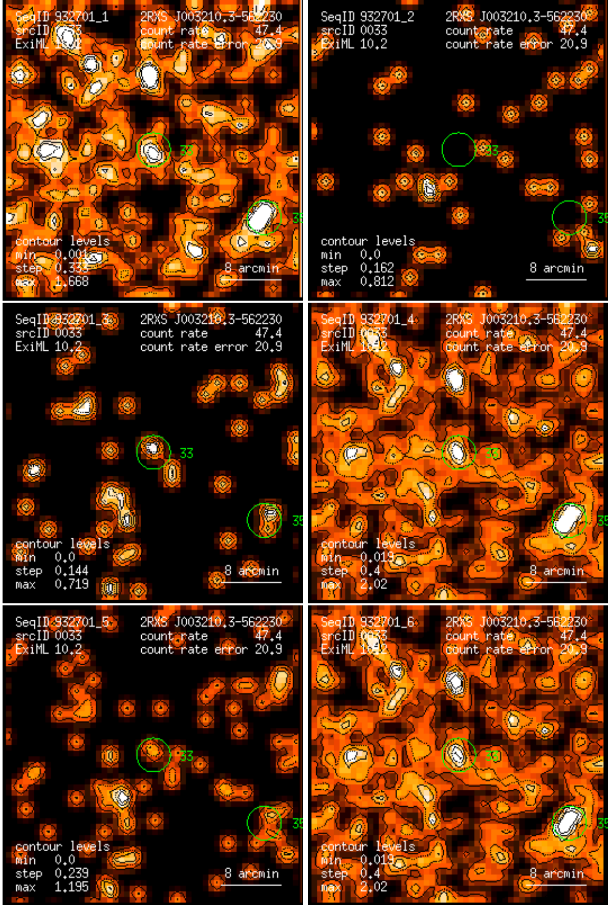
Figure 33: RASS 932701: detection 0033: band rate images, Gaussian filter: (1) PSPC channels 11 – 41, (2) 52 – 90, (3) 91 – 201, (4) 11 – 235, (5) 52 – 201, (6) 11 – 201. Broad band rates in counts/ks. Band rate contour levels in counts/ks/arcmin 2 .
