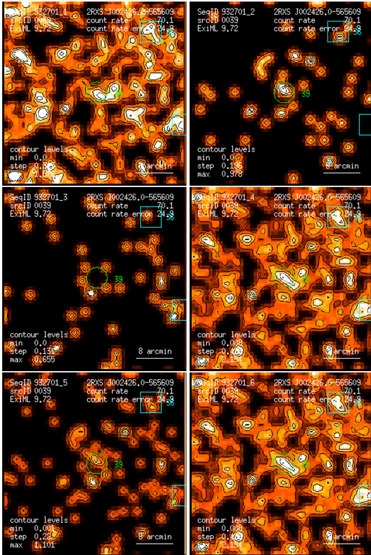
Figure 39: RASS 932701: detection 0039: band rate images, Gaussian filter: (1) PSPC channels 11 – 41, (2) 52 – 90, (3) 91 – 201, (4) 11 – 235, (5) 52 – 201, (6) 11 – 201. Broad band rates in counts/ks. Band rate contour levels in counts/ks/arcmin 2 .
