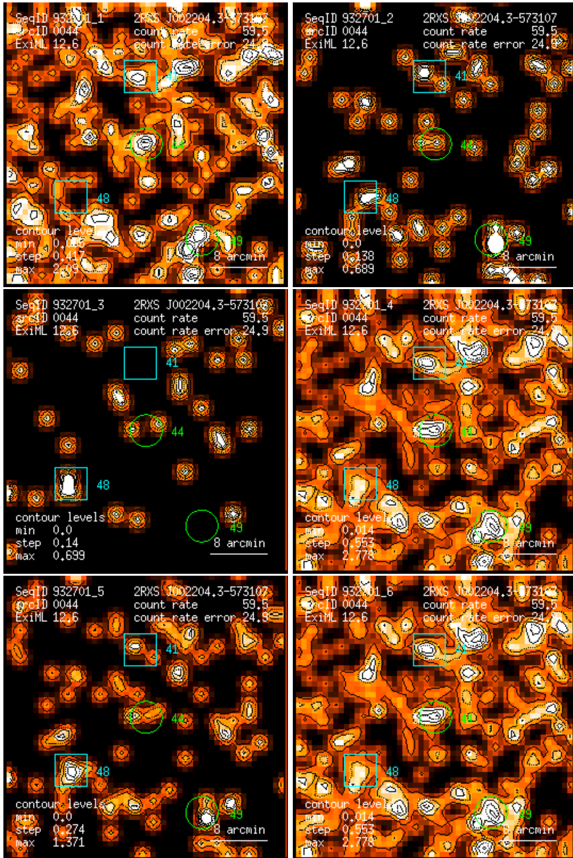
Figure 44: RASS 932701: detection 0044: band rate images, Gaussian filter: (1) PSPC channels 11 – 41, (2) 52 – 90, (3) 91 – 201, (4) 11 – 235, (5) 52 – 201, (6) 11 – 201. Broad band rates in counts/ks. Band rate contour levels in counts/ks/arcmin 2 .
