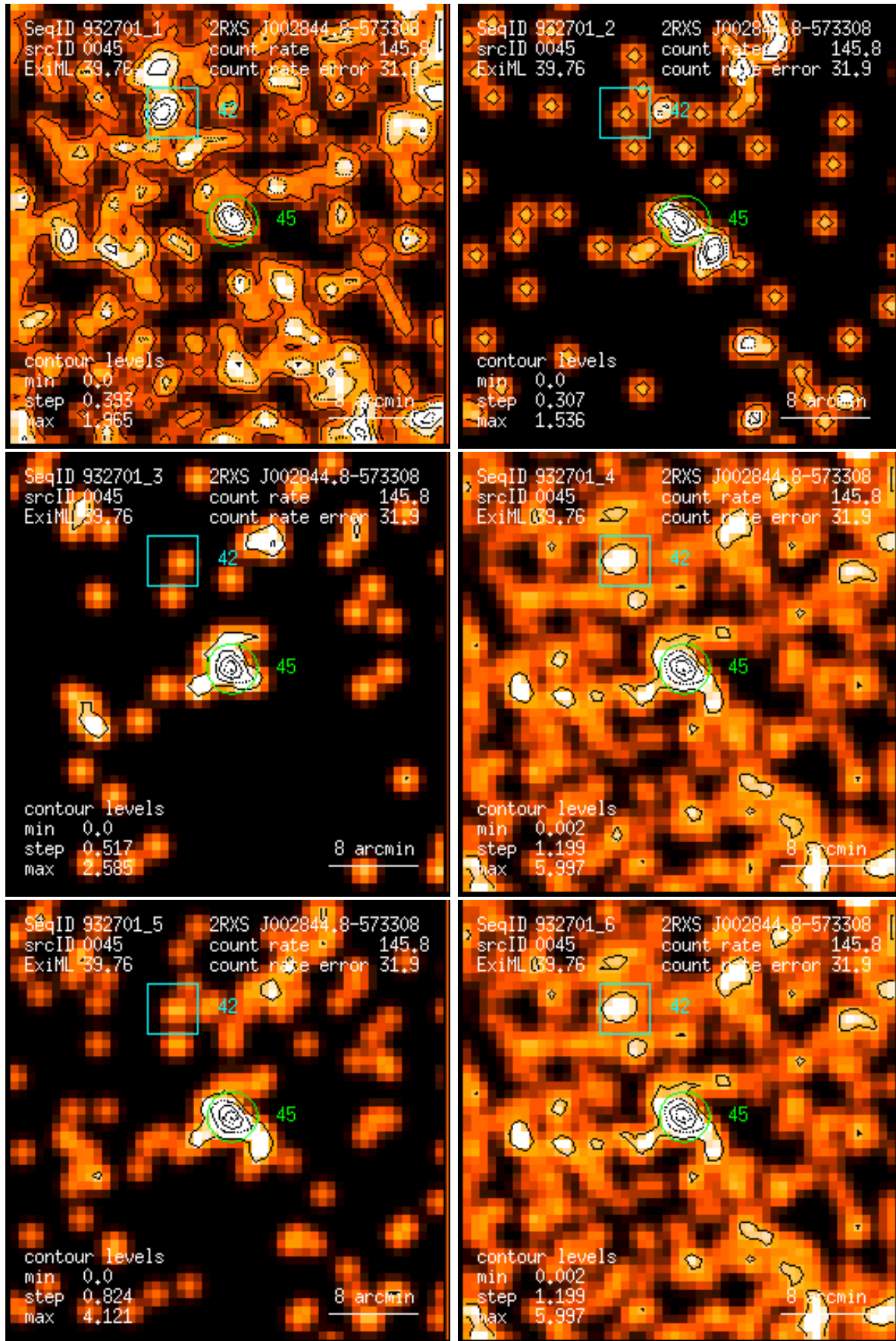
Figure 45: RASS 932701: detection 0045: band rate images, Gaussian filter: (1) PSPC channels 11 – 41, (2) 52 – 90, (3) 91 – 201, (4) 11 – 235, (5) 52 – 201, (6) 11 – 201. Broad band rates in counts/ks. Band rate contour levels in counts/ks/arcmin 2 .
