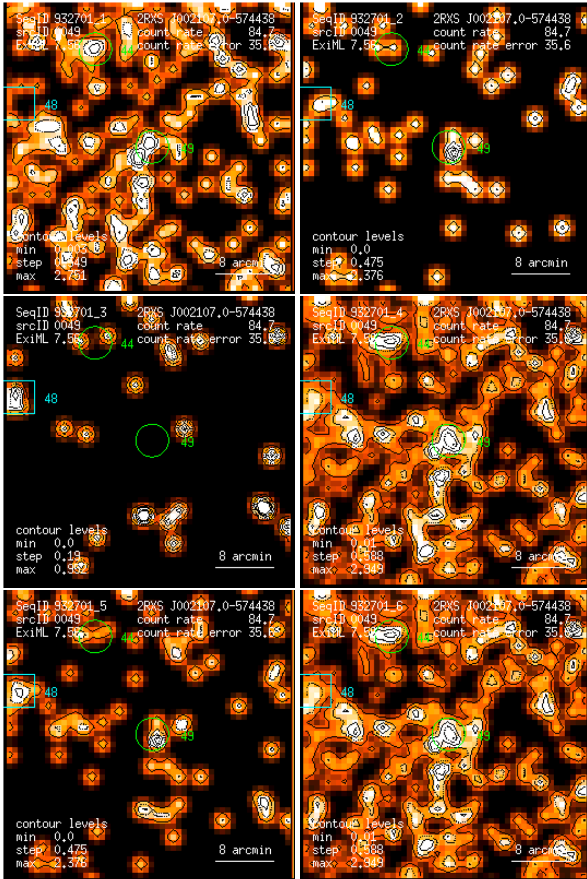
Figure 49: RASS 932701: detection 0049: band rate images, Gaussian filter: (1) PSPC channels 11 – 41, (2) 52 – 90, (3) 91 – 201, (4) 11 – 235, (5) 52 – 201, (6) 11 – 201. Broad band rates in counts/ks. Band rate contour levels in counts/ks/arcmin 2 .
