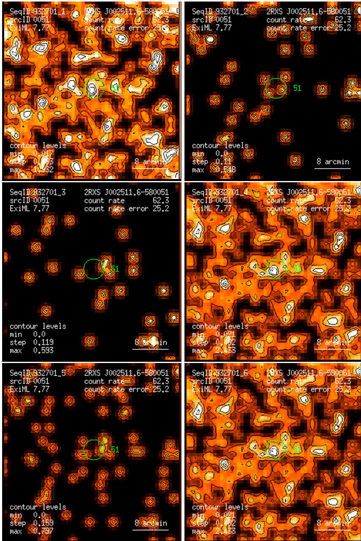
Figure 51: RASS 932701: detection 0051: band rate images, Gaussian filter: (1) PSPC channels 11 – 41, (2) 52 – 90, (3) 91 – 201, (4) 11 – 235, (5) 52 – 201, (6) 11 – 201. Broad band rates in counts/ks. Band rate contour levels in counts/ks/arcmin 2 .
