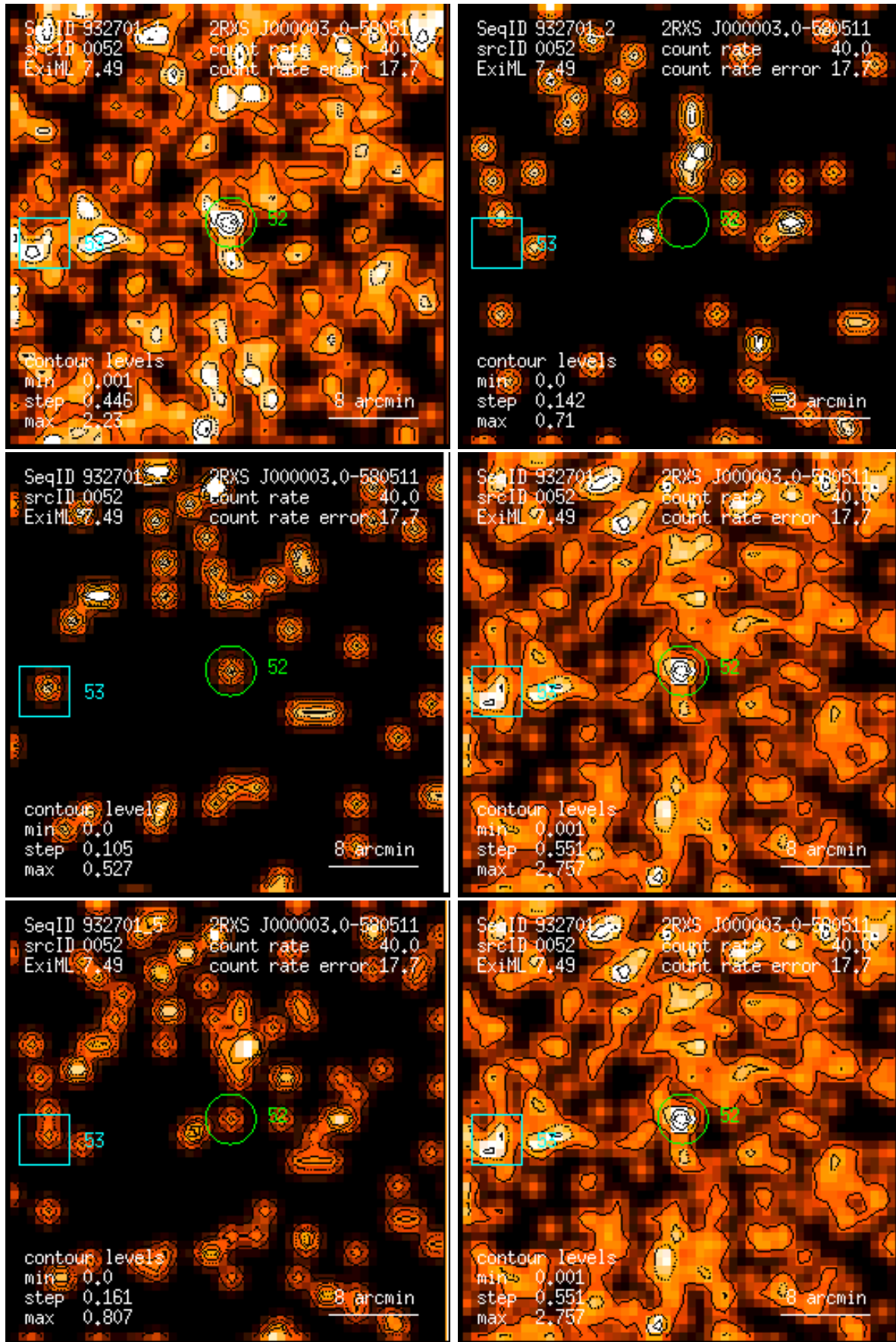
Figure 52: RASS 932701: detection 0052: band rate images, Gaussian filter: (1) PSPC channels 11 – 41, (2) 52 – 90, (3) 91 – 201, (4) 11 – 235, (5) 52 – 201, (6) 11 – 201. Broad band rates in counts/ks. Band rate contour levels in counts/ks/arcmin 2 .
