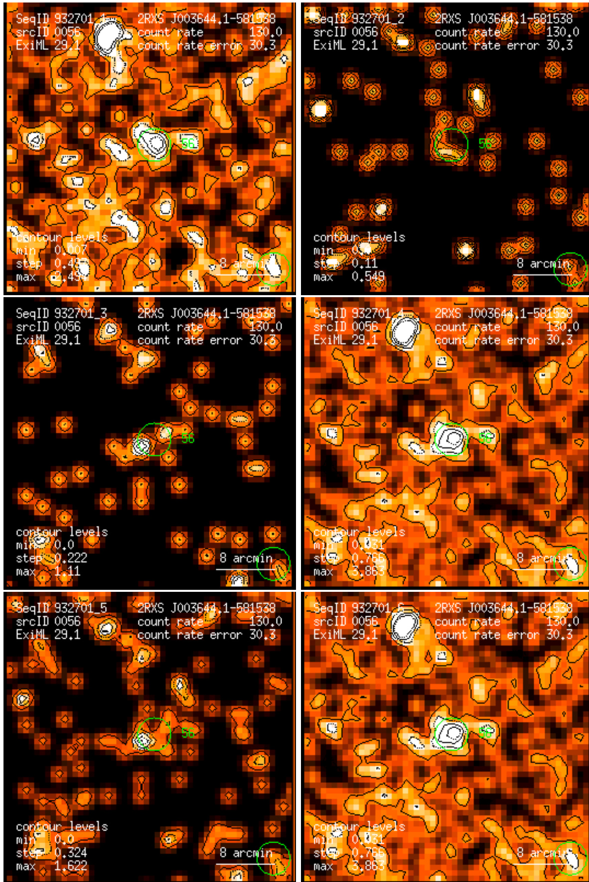
Figure 56: RASS 932701: detection 0056: band rate images, Gaussian filter: (1) PSPC channels 11 – 41, (2) 52 – 90, (3) 91 – 201, (4) 11 – 235, (5) 52 – 201, (6) 11 – 201. Broad band rates in counts/ks. Band rate contour levels in counts/ks/arcmin 2 .
